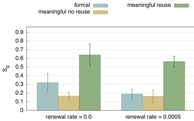
Figure 11. Comparison of strategies. This graph compares the efficiency of the formal marker strategy, the meaningful strategy without reuse, and the reuse strategy for the last 10 games of a run with 5000 games. Left is without population change and right with population change. Average for 50 runs with standard deviation. The reuse strategy is significantly more efficient, even in the case of population turnover. Unsurprisingly, a changing population (shown on the right) makes it harder for the agents to bootstrap an initial system. doi:10.1371/journal.pone.0058960.g011
