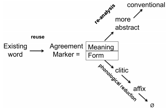
Figure 12. Grammaticalization. Human natural language systems historically build agreement systems by reusing existing words. The form of these words then undergoes erosion by phonological reduction processes until the marker may get lost entirely. Their meaning becomes more abstract and semantic features become purely conventional rather than grounded in the meaning of the word, through coercion. doi:10.1371/journal.pone.0058960.g012
