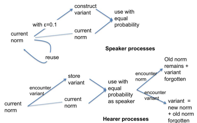
Figure 13. Phonological reduction strategy. Speakers construct a new variant by phonologically reducing a marker’s form with a probability \epsilon=0.1 . The hearer is able to recognize a variant if it deviates only for one consonant or vowel and will adopt it as the new norm for the marker when the variant is encountered twice. doi:10.1371/journal.pone.0058960.g013
