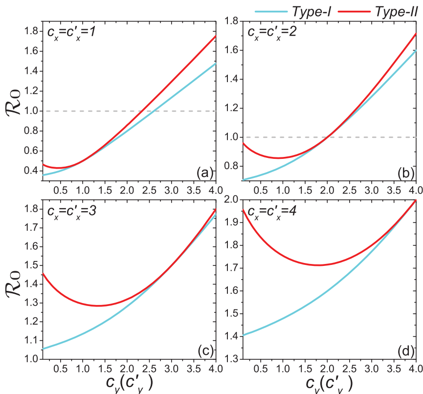
Figure 6 | Comparison of the phase diagrams of global \mathcal{R}_0 between the type-I and type-II contact scenarios. Each panel shows the variance of global \mathcal{R}_0 as c_y ( c'_y ) gradually increases, with c_x = c'_x = 1 in (a), c_x = c'_x = 2 in (b), c_x = c'_x = 3 in (c), c_x = c'_x = 4 in (d). The horizontal gray dashed lines in the upper two panels illustrate the threshold value \mathcal{R}_0 = 1 .
