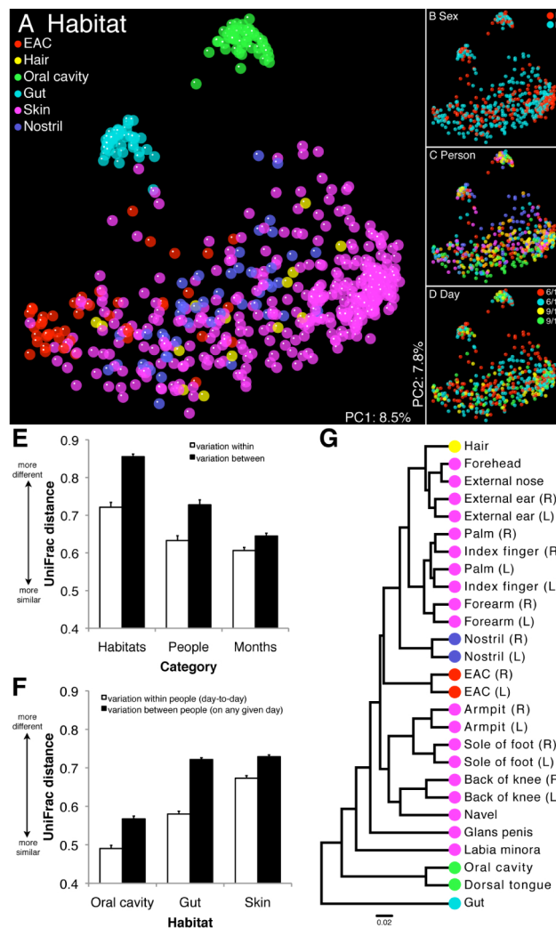
Fig. 1. 16S rRNA gene surveys reveal hierarchical partitioning of human-associated bacterial diversity. (A to D) Communities clustered using PCoA of the unweighted UniFrac distance matrix. Each point corresponds to a sample colored by (A) body habitat, (B) host sex, (C) host individual, or (D) collection date. The same plot is shown in each panel. F, female; M, male. (E and F) Mean ( \pm SEM) unweighted UniFrac distance between communities. In (E) habitats are weighted equally and in (F) skin comparisons are within sites. (G) UPGMA clustering of composite communities from the indicated locales. Leaves are colored according to body habitat as in (A). R, right; L, left.
