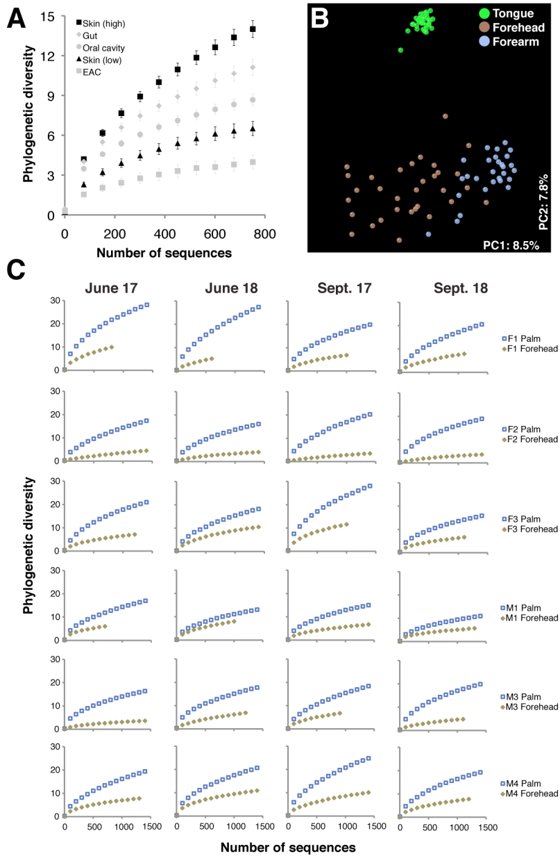
Fig. 2. Site-to-site variation on skin surfaces. (A) Rarefaction curves for communities sampled from skin and other habitats. Phylogenetic diversity is in units of branch length. Mean \pm 95% confidence interval shown. (B) PCoA plot as in Fig. 1 showing only dorsal tongue, forehead, and volar forearm samples. (C) Individual rarefaction curves for forehead and palm communities.
