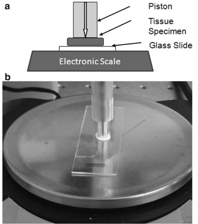
FIG. 1. (a) Schematic side view of the compression system used to measure indentation of soft tissue samples. The large white arrow shows the motion direction of the piston. (b) Photograph of the compression system testing a tissue specimen placed on top of a glass slide (arrow). The diameter of the compression piston is 1.0 cm.
