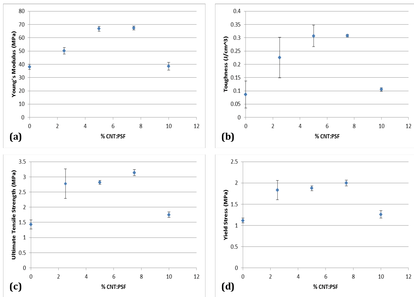
Figure 4 | Plots of (a) Young's modulus (MPa), (b) Toughness ( \text{J}/\text{cm}^3 ), (c) Ultimate tensile strength (MPa) and (d) Yield Stress (MPa) as a function of CNT loading in PSF. At a concentration of 7.5% CNTs in the polymer composite, there is a 119% increase in the ultimate tensile strength, 77% increase in the Young's modulus, 258% increase in the toughness and a 79% increase in the yield strength. These increases are relative to 0% CNT loading.
