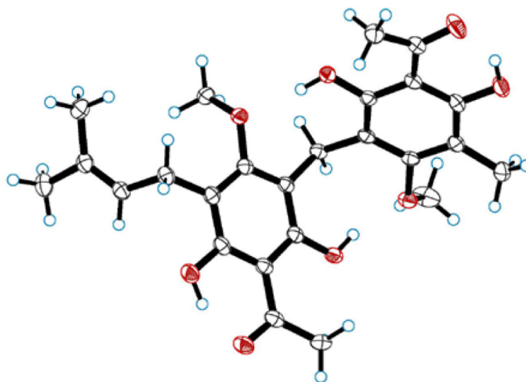
Figure 2. Anisotropic displacement ellipsoid drawing (50%) of 1 .
