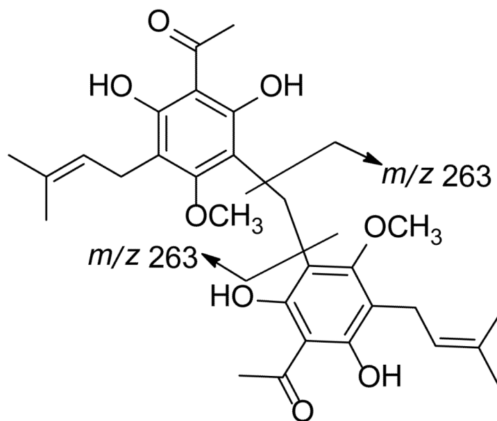
Figure 3. Mass fragmentation observed for 2.
