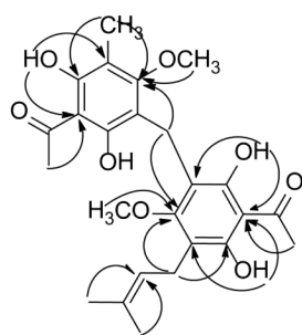
Figure 1. Important HMBC correlations observed in 1 .
