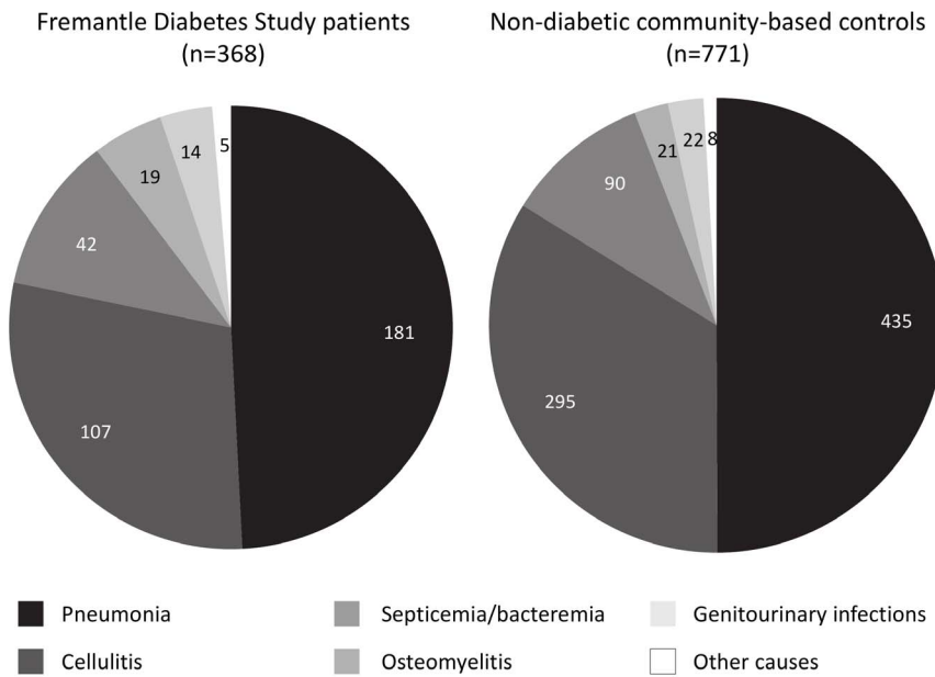
Figure 1. Pie graphs showing the numbers of bacterial infections necessitating hospitalization by type for diabetic patients (left panel) and matched non-diabetic controls (right panel). doi:10.1371/journal.pone.0060502.g001
