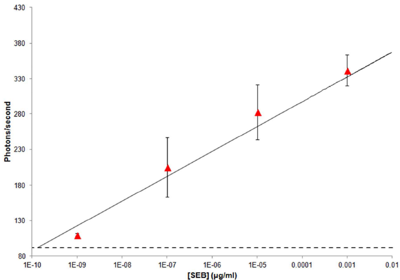
Figure 5. Measured results of SEB in milk (▲) compared to the standard curve (solid line, R^2 : 0.96) of SEB in PBS. Final concentrations after 100-fold dilution with buffer were 10^{-9} , 10^{-7} , 10^{-5} and 0.001 µg/mL. Error-bar: standard deviation determined from five replicates.
