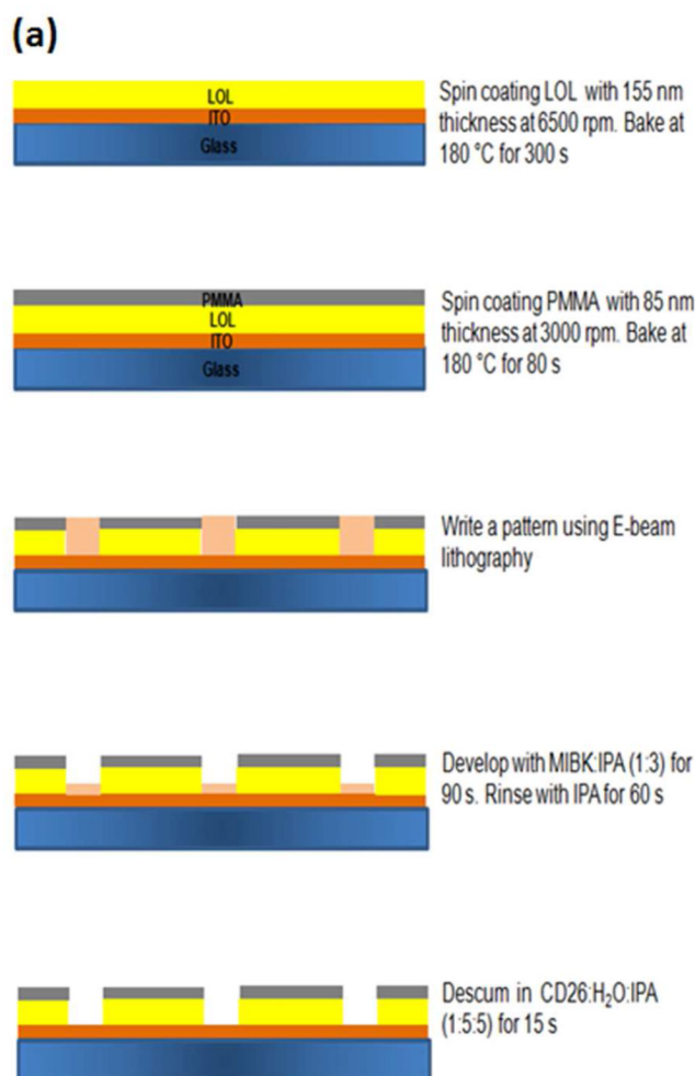
Figure 2. Photonics crystal (PC)-nanowells/array. (a) fabrication of PC-nanowells/array and (b) scanning electron microscope (SEM) image of the PC-nanowells/array; width of the well: 60 nm; periodicity: 350 nm; coating thickness: 240 nm (85 nm-PMMA and 155 nm-LOL), white dashed line: signal collecting area (25 μm×25 μm) by a single photon counting detection system.
