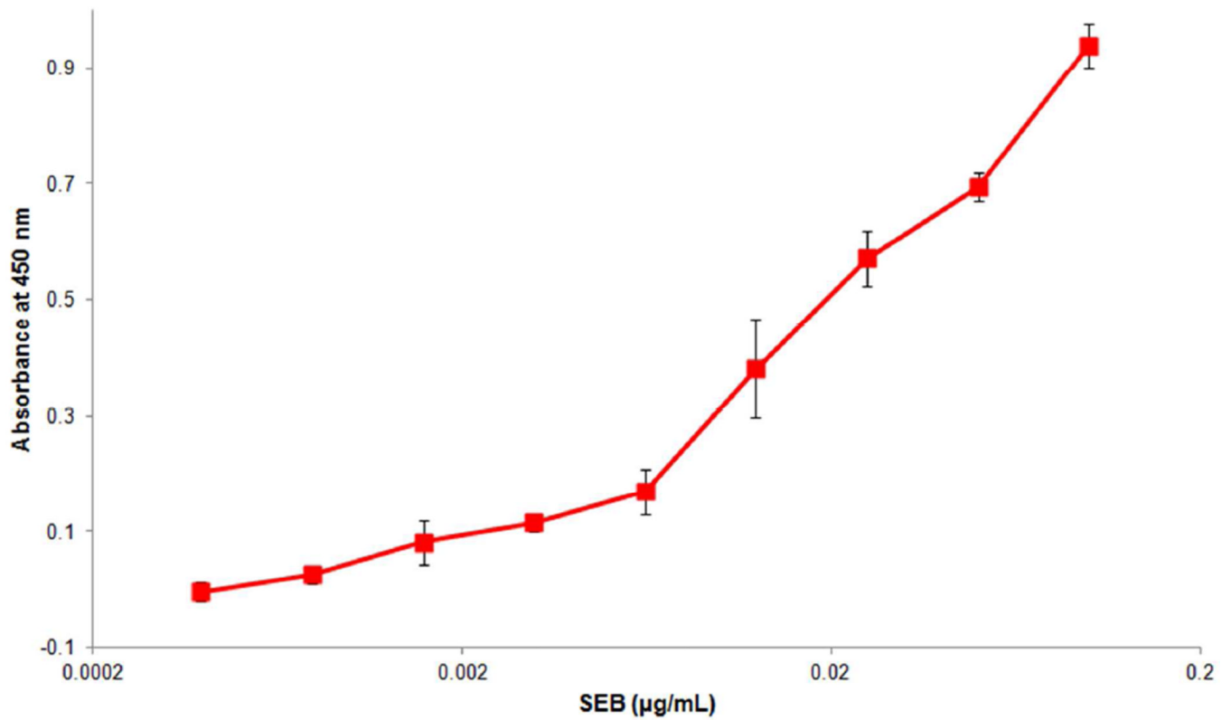
Figure 4. Detection of SEB using conventional 96-well plate-ELISA; Absorbance test using HRP and substrate. Concentrations of 0 , 4 \times 10^{-4} , 8 \times 10^{-4} , 16 \times 10^{-4} , 31 \times 10^{-4} , 63 \times 10^{-4} , 125 \times 10^{-4} , 25 \times 10^{-3} , 0.05 , 0.1 µg/mL. LOD was 10^{-3} µg/mL. Error bars represent one standard deviation based on four replicates.
