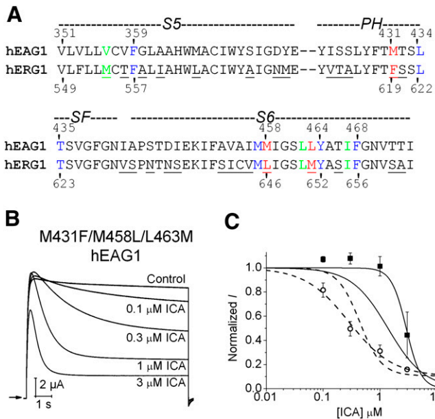
Fig. 5. ICA induces inactivation of mutant hEAG1 channel with putative drug-binding pocket engineered to mimic hERG1 channel. (A) Amino acid sequence alignment of S5 and pore helix (PH)/selectivity filter (SF)/S6 region of hEAG1 and hERG1. Nonconserved amino acids are underlined. Conserved residues (blue) and nonconserved residues (red) predicted to line the hydrophobic ICA binding pocket in hERG1 are highlighted. Residues colored green were predicted to contribute to ICA binding site in closed state of hEAG1 (but not predicted to interact with hERG1 in closed or open state). (B) Concentration-dependent inhibition of M431F/M458L/L463M hEAG1 channel currents by ICA. Currents were elicited with 10-second pulses to +30 mV. (C) [ICA]-response relationships for I_{\text{peak}} (solid curve) and I_{\text{end}} (dashed curve) quantified as fold change in current measured at a test potential of +30 mV for M431F/M458L/L463M (data points, ■ and ○) and WT hEAG1 (curves only, replotted from Fig. 1C). The IC_{50} was 0.49 \pm 0.15 \mu\text{M} for I_{\text{end}} and 2.96 \pm 0.82 \mu\text{M} for I_{\text{peak}} ( n = 4 ).
