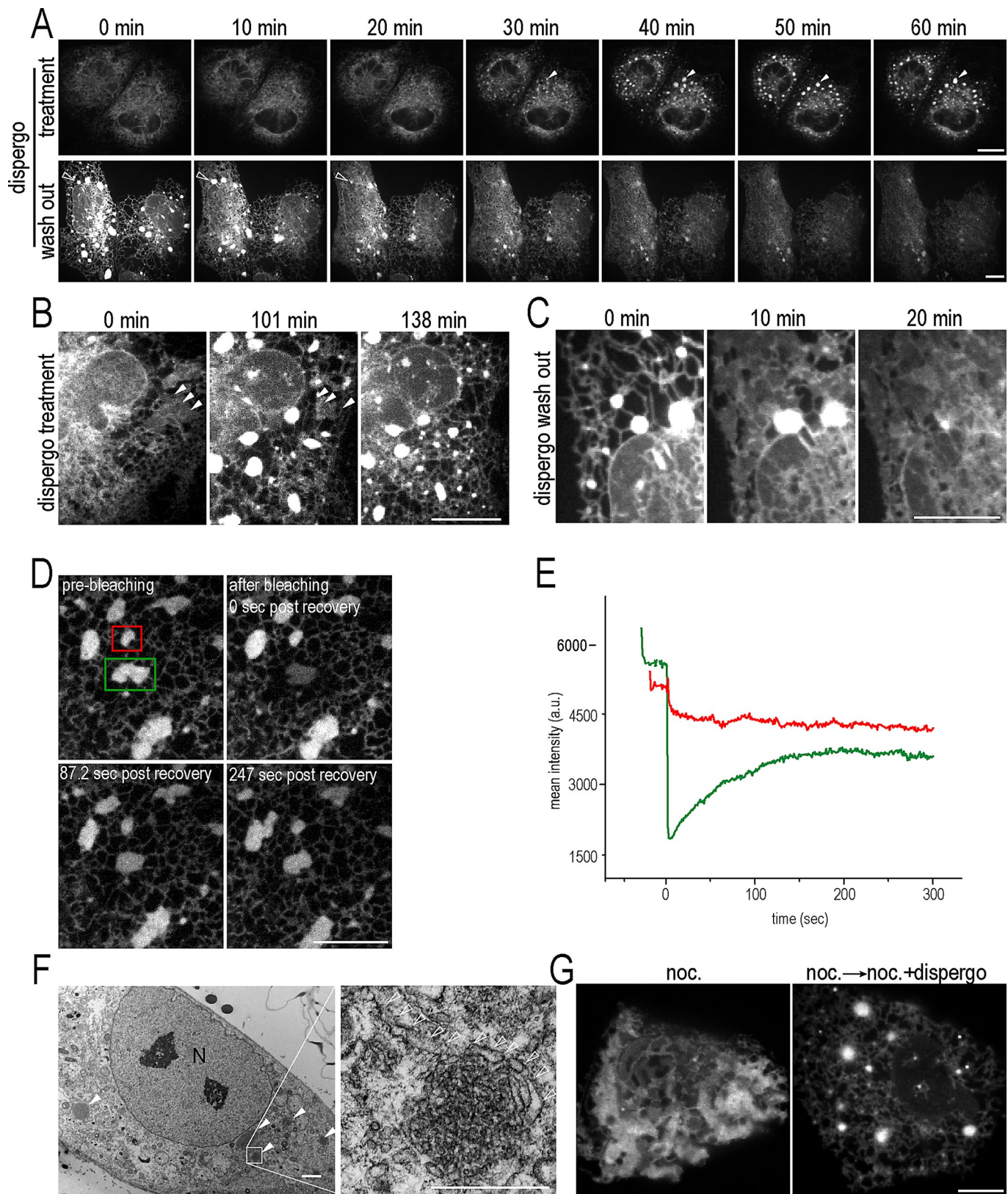
FIGURE 3: Effect of dispergo on the dynamics and morphology of the ER. (A) The effects of dispergo are reversible. Two-dimensional time-lapse series of BSC1 cells stably expressing GFP-Sec61 \beta treated with dispergo for 1 h, showing the gradual appearance of ER patches (top, solid arrowheads; see Supplemental Movie S1). After a further 2-h incubation with dispergo, the compound was removed (bottom). The time-lapse series shows the gradual disappearance of the ER patches (bottom, open arrowheads; see Supplemental Movie S2). (B, C) Two-dimensional time-lapse series from BSC1 cells expressing mRFP1-Sec61 \beta (B) or GFP-Sec61 \beta (C). The images in B highlight the disappearance of ER cisternae (arrowheads) and appearance of ER patches upon dispergo treatment. The images in C are from an enlarged
