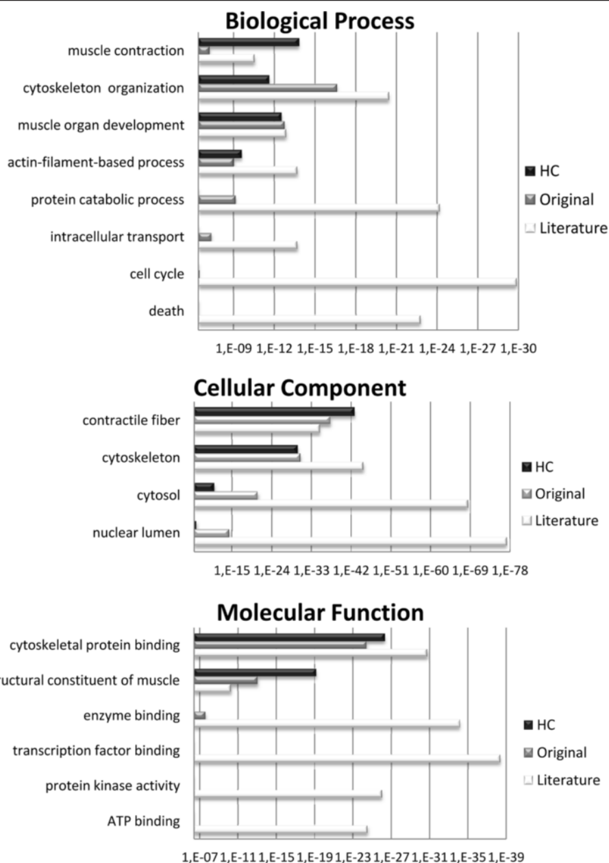
Figure 7 GO enrichment analysis of the three datasets compared to the human proteome. A GO term enrichment analysis of the three datasets (LGMD-centred, HC and literature-enriched datasets) was performed using the DAVID web-resource and an appropriate level of abstraction of the annotations. The bar charts depict enriched GO terms of the three datasets compared to the human proteome in the three branches of the GO structure as a function of the EASE score.
