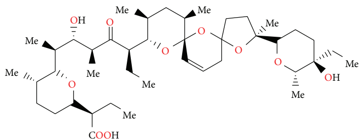
FIGURE 41: Structure of SY-1.
