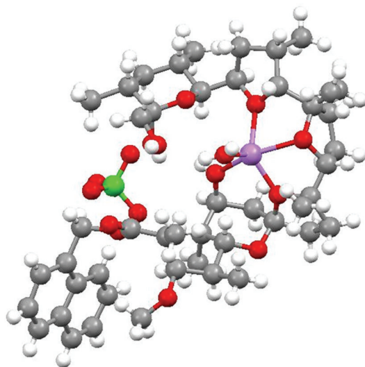
FIGURE 56: Crystal structure of monensin 1-naphtylmethyl ester with the lithium perchlorate.
