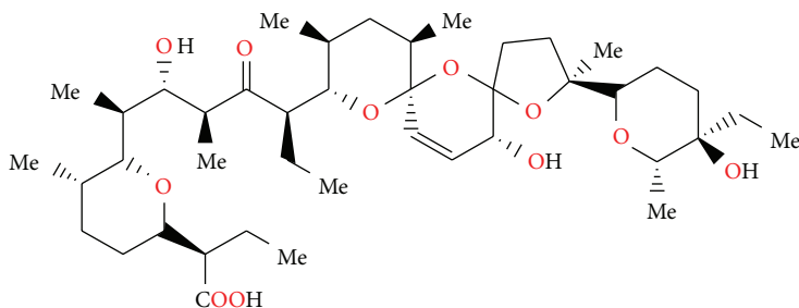
FIGURE 42: Structure of SY-2.
