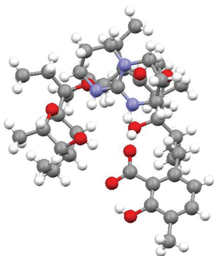
FIGURE 31: Crystal structure of lasalocid complex with TBD.
