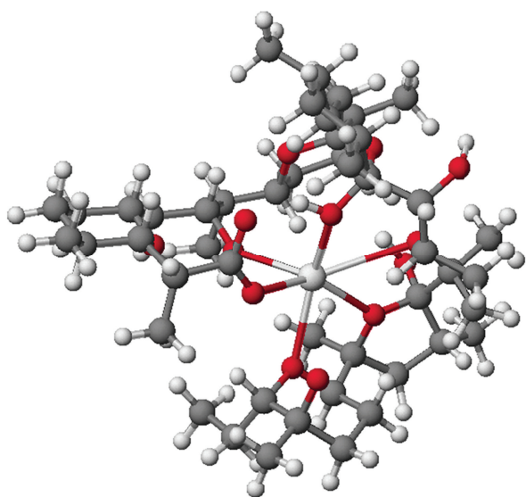
FIGURE 2: Structure of 6-demethyl-alborixine complex with sodium cation.
