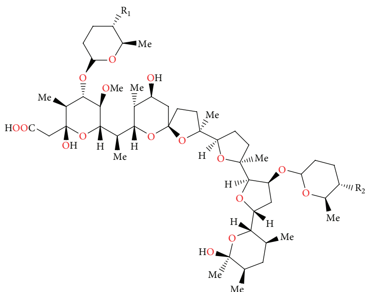
FIGURE 60: Structure of octacyclomycin.
