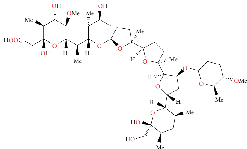
FIGURE 33: Structure of CP-120509.
