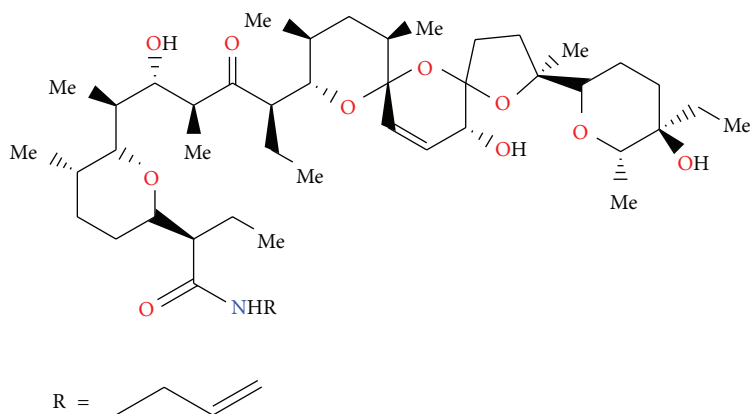
FIGURE 48: Structure of allyl amide of salinomycin.
