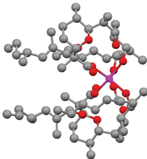
FIGURE 36: Crystal structure of zincophorin magnesium salt.
