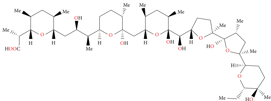
FIGURE 1: Structure of alborixine.
