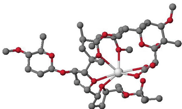
FIGURE 4: Crystal structure of antibiotic 6016 thallium salt.
