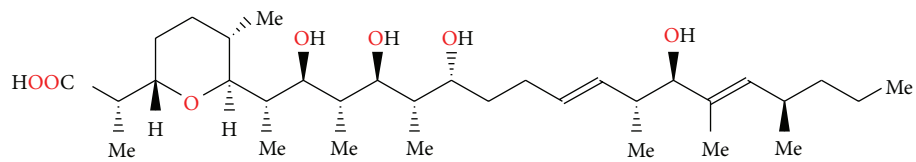
FIGURE 35: Structure of zincophorin.
