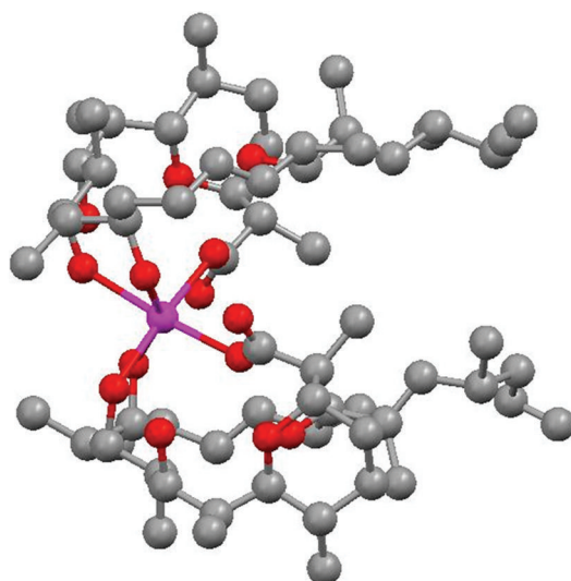
FIGURE 38: Crystal structure of CP-78545 cadmium salt.
