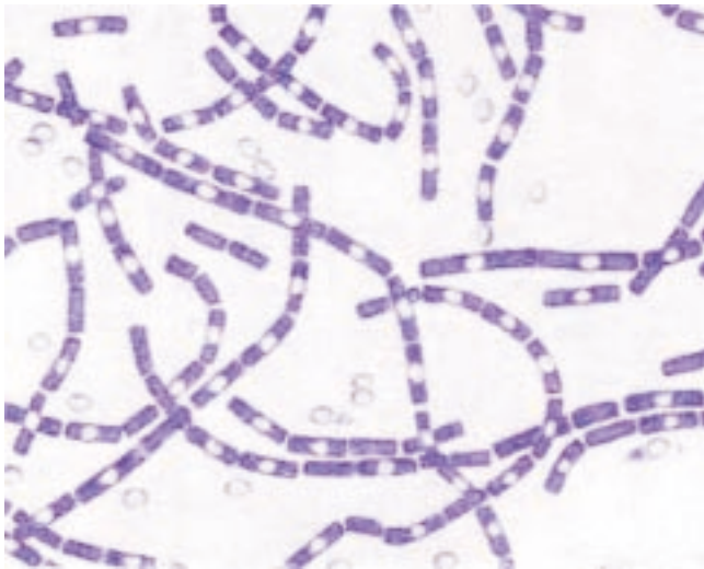
Figure 1. Characteristics of B. anthracis . Gram stain (1 500 \times ).
