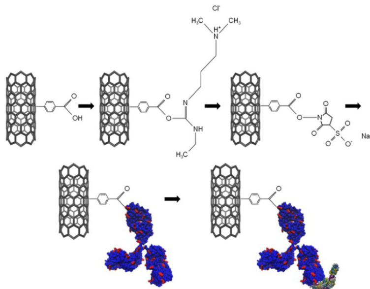
Figure 1. Functionalization chemistry for Lyme antibody and binding of flagellar antigen. First, a pristine nanotube is treated with diazonium salts to create sp^3 hybridization sites ending in carboxylic acid moieties. The carboxylic acid is activated with EDC and stabilized with sulfo-NHS. The sulfo-NHS is displaced by the primary amine in a surface lysine residue (depicted in red) on the anti-p41 antibody. The flagellar antigen (depicted according to secondary structure in purple, cyan, and yellow) then binds to the epitope on the antibody during the exposure step.
