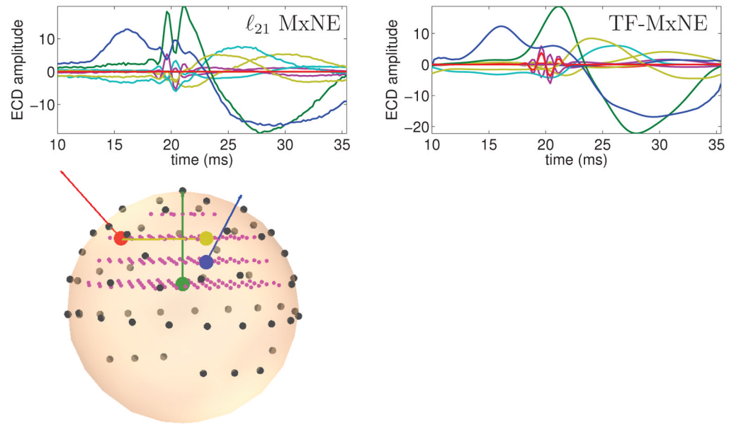
Figure 5. Results with real EEG lead field (SNR=3dB). The 4 dipoles are color coded. Magenta dots show the 3D grid of sources. Dark dots show the EEG sensors locations. Contrary to TF l_{21} + l_1, l_{21} fails to recover the deep green dipole time course.
