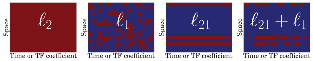
Figure 2. Sparsity patterns promoted by the different priors: l_2 all non-zero, l_1 scattered and unstructured non-zero, l_{21} block row structure, and l_{21} + l_1 block row structure with intra-row sparsity. Red color indicates non-zero coefficients.
