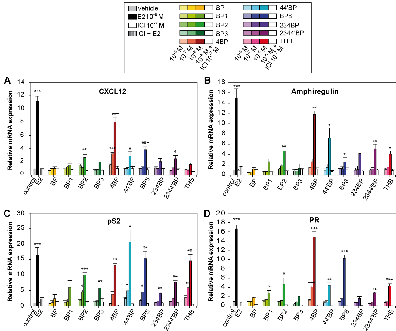
Figure 3. Evaluation of BP-induced expression of several endogenous estrogen-regulated genes. After hormone deprivation for 24 h, MCF-7 cells were grown in medium containing 2.5% dextran-treated charcoal stripped FBS and treated with 10 -8 M E2 or different concentrations of BPs (10 -8 , 10 -7 and 10 -6 M, illustrated by color gradations) for 48 h. In addition, treatments to 10 -6 M BPs were also performed in presence of 10 -7 M of the anti-estrogen ICI 182,780 (ICI) (open bars for BP + ICI treatments and hatched bar for E2 + ICI treatment). The expression levels of several E2-regulated genes, (A) CXCL12, (B) Amphiregulin, (C) pS2 and (D) Progesterone Receptor (PR), after the treatments were quantified using real-time PCR. Data are the mean values from triplicate experiments \pm SEM (* P < 0.05, ** P < 0.01, *** P < 0.001). doi:10.1371/journal.pone.0060567.g003
