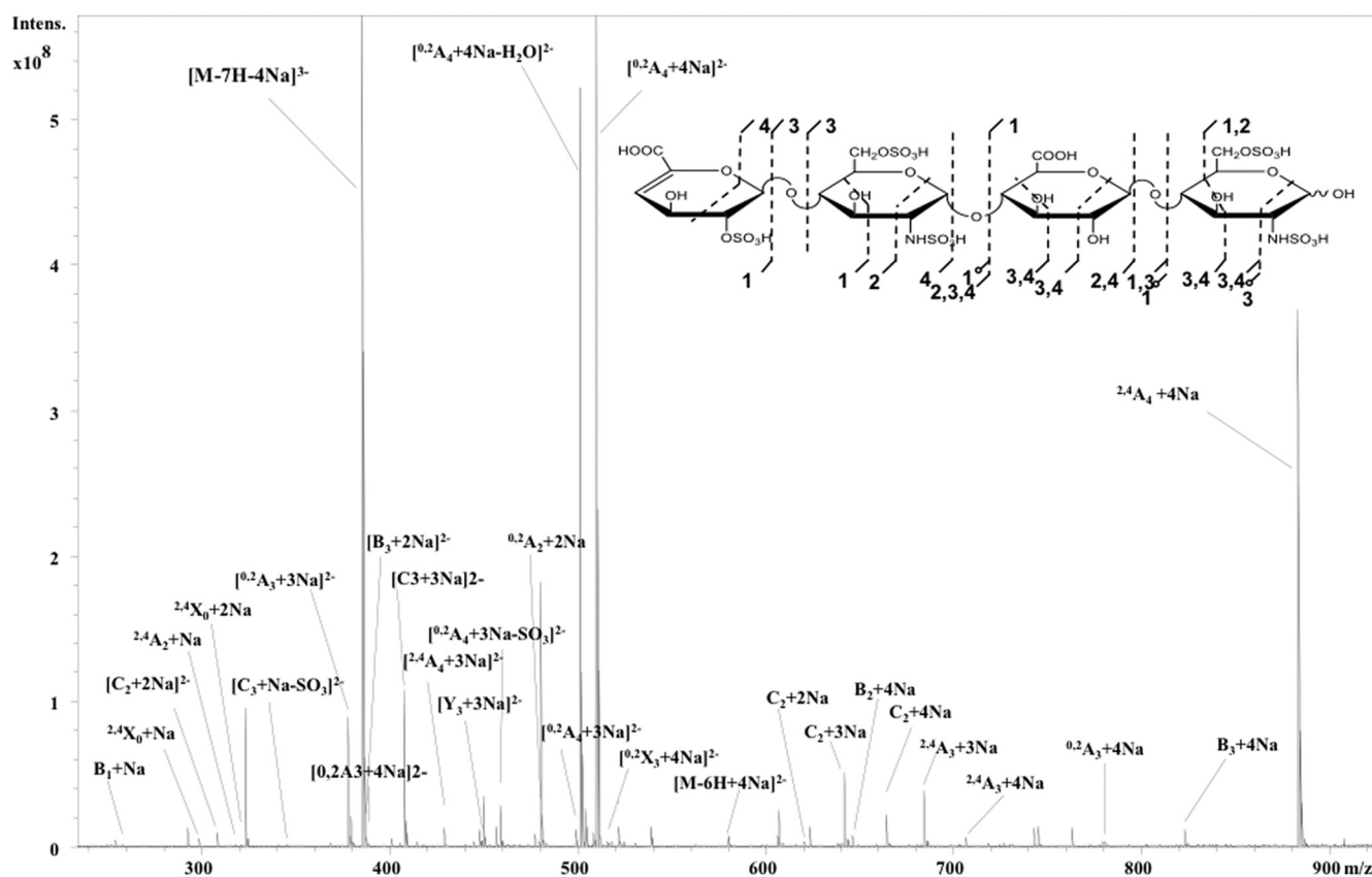
FIG. 1. CID spectra of penta-sulfated heparin tetramer, precursor [M - 7H + 4Na]^{3-} . The fragment ions observed are shown in the annotated structure ( inset ). The precursor used has all the sulfates and carboxyl groups ionized through charge or Na^+/H^+ exchange.
