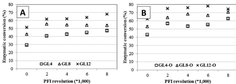
Figure 7 Enzyme hydrolysis improvement through the use of mechanical refining alone (7a) and refining + oxygen delignification (7b). Enzyme hydrolysis efficiency based on carbohydrate content in pretreated substrate (77%). From Koo [13]. GL = Green Liquor Pretreatment”. GL-4 = “Green Liquor Pretreatment with 4% Total Titratable Alkali”. GL-4-O = “Green Liquor Pretreatment with 4% Total Titratable Alkali + Oxygen Delignification”.
