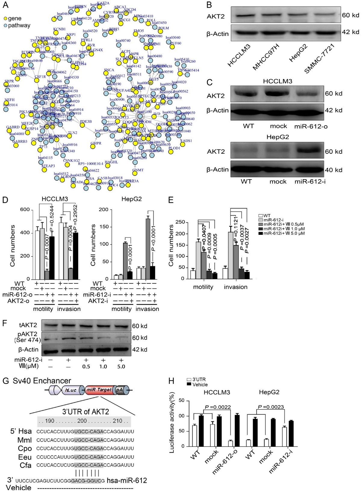
Figure 5. Direct regulation of miR-612 on AKT2 expression. (A) Bioinformatics analysis to predict target gene of miR-612 and assay pathway perturbation. (B) Western blot analysis to quantify endogenous levels of AKT2 in HCCLM3, MHCC97H, HepG2, and SMMC-7721 cells. (C) Protein levels of AKT2 in HCCLM3 and HepG2 cells after indicated treatments were detected by Western blots. (D) Motility and invasion assays for HCCLM3 (left) and
