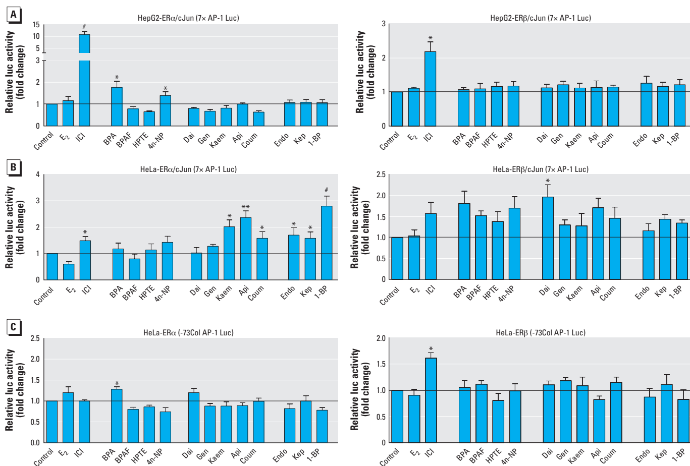
Figure 3. EDCs act as agonists on ER \alpha and ER \beta to activate the tethered mechanism (AP-1). (A) Effects of EDCs on ER \alpha 7×AP-1 Luc reporter activity in HepG2 (top) and HeLa (bottom) cells transfected with 7×AP-1 Luc, pRL-TK, pcDNA/WT-ER \alpha or -ER \beta , and pRSV/c-Jun plasmids overnight and then treated with vehicle (control), 10 nM E 2 , 100 nM ICI, or EDCs for 18 hr; ER AP-1-mediated activation was detected by luciferase reporter assays. (B) Effects of EDCs on ER \alpha - and ER \beta -73Col AP-1 Luc reporter activity in HeLa cells transfected with -73Col AP-1 Luc, pRL-TK, and pcDNA/WT-ER \alpha or -ER \beta plasmids overnight and then treated with vehicle (control), 10 nM E 2 , 100 nM ICI, or EDCs for 18 hr; ER-73Col AP-1-mediated activation was detected by luciferase reporter assays. See “Materials and Methods” for details of the experiments. Data shown represent mean fold change ( \pm SE) relative to the control.
