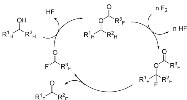
Scheme 11. The PERFECT method for synthesis of perfluoro ketones.
