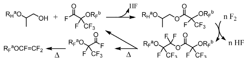
Scheme 8. The PERFECT method for synthesis of various perfluorinated acyl fluorides.
