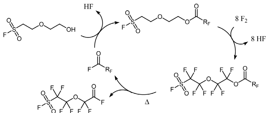
Scheme 10. The PERFECT method for synthesis of monomers for perfluorosulfonic acid membrane.
