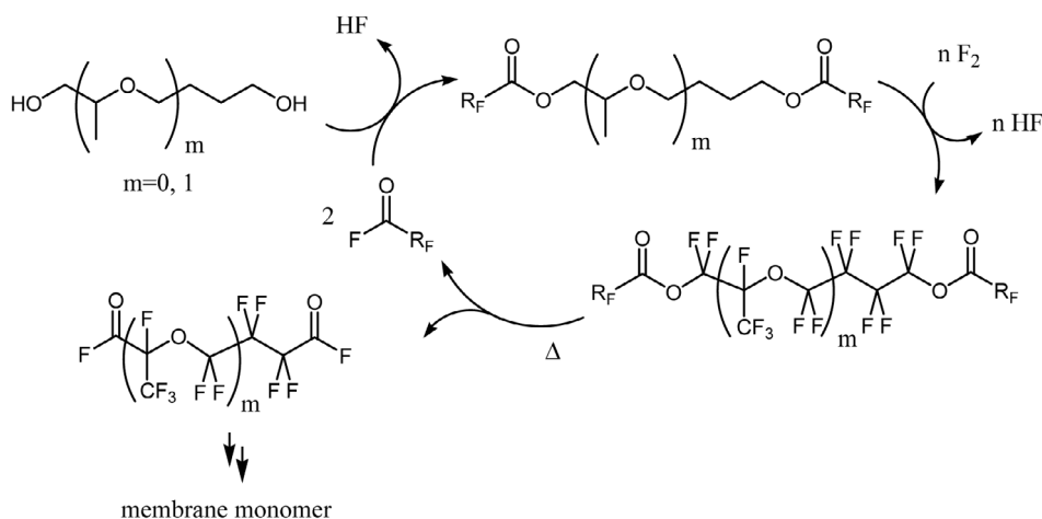
Scheme 9. The PERFECT method for synthesis of monomers for carboxylic acid membrane.
