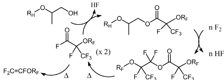
Scheme 7. The PERFECT method for synthesis of perfluorinated vinyl ethers.
