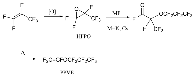
Scheme 3. Synthesis of PPVE.
