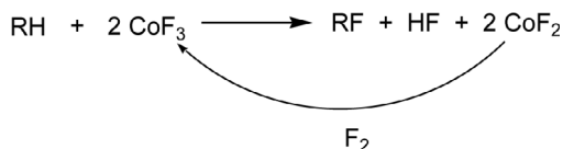
Scheme 1. Fluorination with \text{CoF}_3 .
