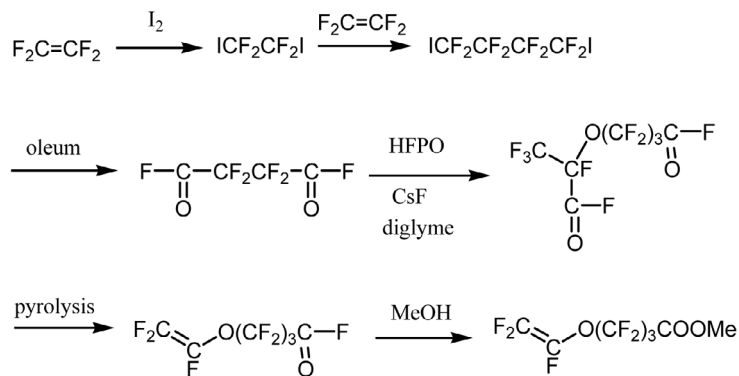
Scheme 5. Synthesis of a monomer for perfluorinated carboxylic acid membrane.
