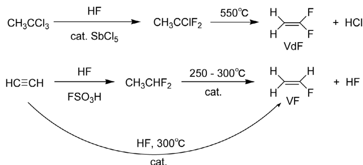
Scheme 2. Synthesis of partially-fluorinated ethylene monomers.
