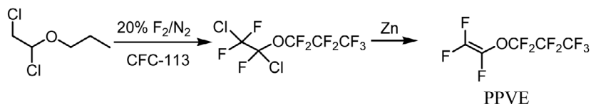
Scheme 6. Synthesis of PPVE from a non-fluorinated dichloroethyl ether.
