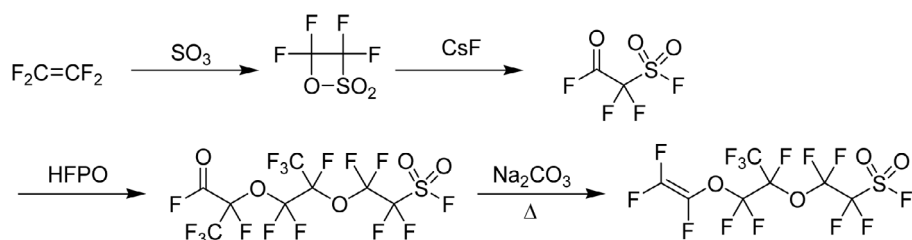
Scheme 4. Synthesis of a monomer for ion-exchange membrane.
