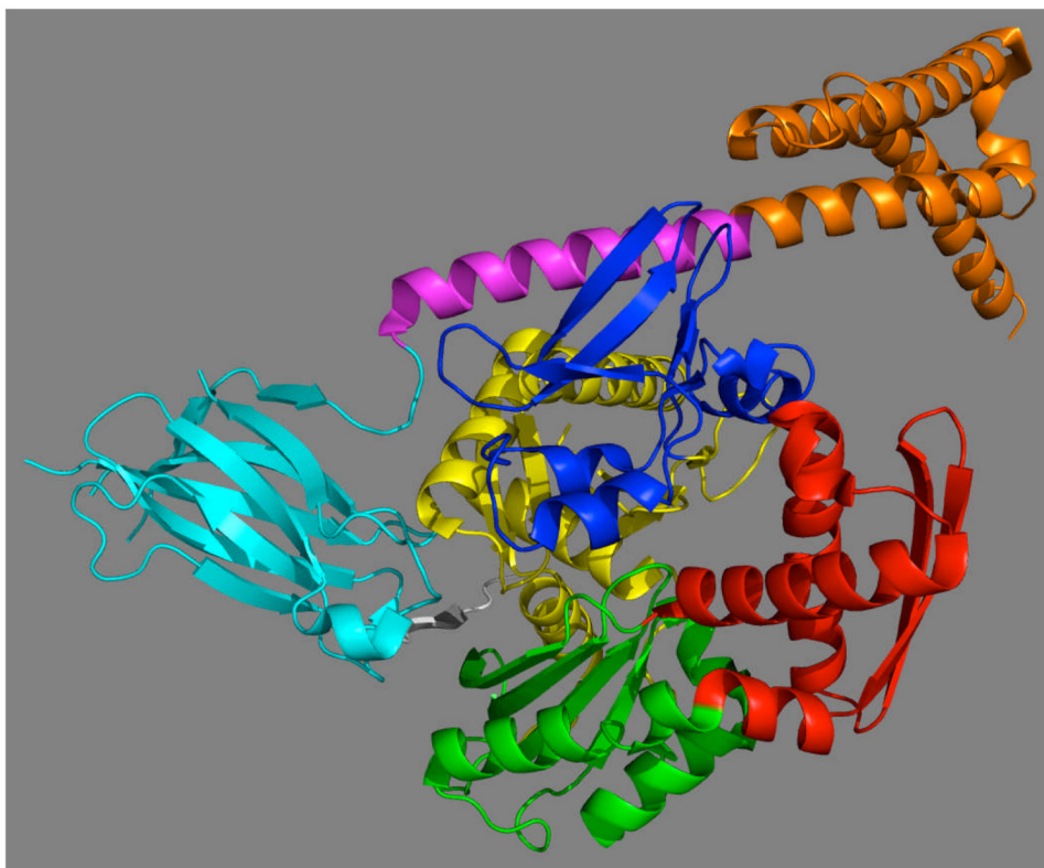
Figure 5. A crystal structure of Hsp110 of S. cerevisiae 81 Orientation and color coding is as in Fig 3a. (NBD domain IA: yellow, IB: blue, IIA: green, IIB: red, linker: white, beta domain: cyan, LID-helix-A: magenta, LID-helix-B: pink, Lid: orange).
