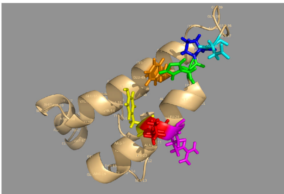
Figure 16. The solution structure of E. coli DnaJ(2-76) in context of DnaI(2-108) (1XBL) 212 . The mutationally sensitive 213 residues Y25 (yellow), K26 (red), R26 (magenta), H33 (green), P34 (blue), D35 (cyan) and F47 (orange) are high-lighted.
