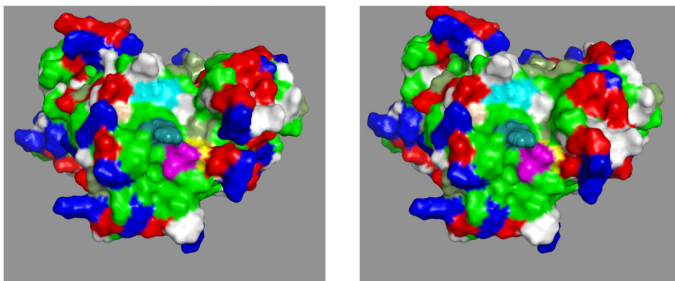
Figure 8. The SBD's view of the IA / IIA interface of DnaK-TTh . A, Left: in the ADP state. B, Right: in the AMPPNP state 83 . Color coding: hydrophobics, green; positive, blue; negative, red; polar, white. The C-terminus (residue 372) is magenta. Residue L174 (L177 in DnaK E. coli ) in yellow, residue R148 (R151 in E. coli ) in cyan, residue A152 (K155 in E. coli ) sand, residue R164 (R167 in E. coli ) in teal.
