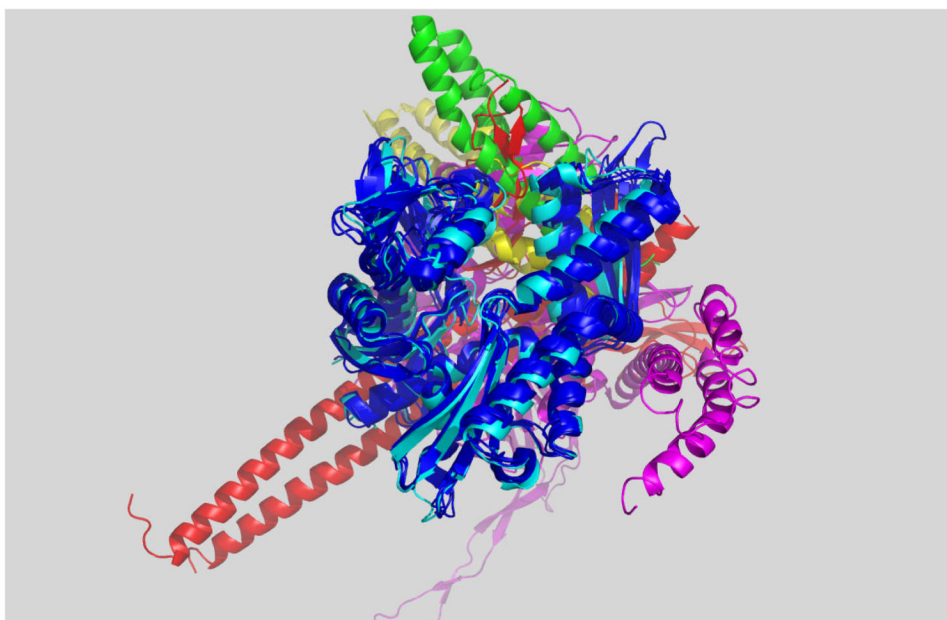
Figure 14. NBD-NEF complexes. The NBD's were superposed and all colored blue. GrpE (1DKG) in red; Hsp110 (3C7N) in magenta, BAG-1 (1HX1) in green; BAG-2 (3CQX) in yellow. The NBD of HSC without NEF (3HSC) is shown in cyan.
