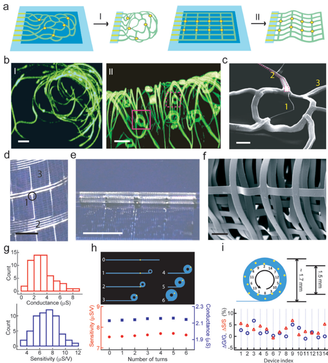
Figure 2. Macroporous and flexible nanowire nanoES
