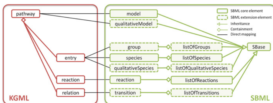
Figure 3 Simplified class structure and mapping from KGML to SBML. This mapping includes the SBML qualitative models (qual) and groups extension packages. Most properties are encoded as attributes on the actual classes. Tables 1 and 2 give further details about translation of entries and relations. SBML can only handle reactions. Therefore, SBML-qual is required to properly encode relations. This extension package requires its own model. Subsequently, the SBML-core model and each species have to be duplicated to obtain a qualitativeModel including the translated relations. Furthermore, the groups extension package can be used for a proper encoding of groups in SBML.
