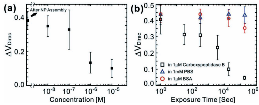
Figure 4. Enzyme detection using the graphene-nanoparticle hybrid sensor (a) Sensitivity ( \Delta V_{Dirac} ) of the graphene sensor as a function of enzyme concentration [ n = 10 ]. (b) \Delta V_{Dirac} change under various periods of exposure to a 1 \mu\text{M} solution of Carboxypeptidase B in PBS (black square), a 1 \text{mM} PBS solution (blue triangle) and 1 \mu\text{M} solution of BSA in the PBS (red circles) [ n = 10 ].
