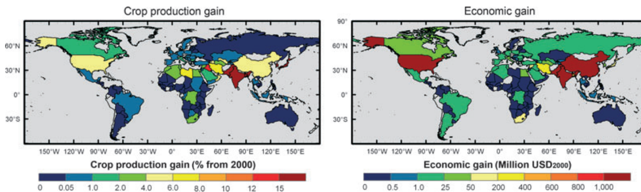
Fig. 3 Total (soybean, maize, and wheat) year 2030 crop production (CP) gain in each nation due to cultivating O_3 tolerant crops ( CLE_{min} ) relative to the median sensitivity of cultivars analyzed in US field studies ( CLE_{med} ), represented as a percent increase from year 2000 production (left). The estimated economic value (EV) of CP gains is also shown (right).
