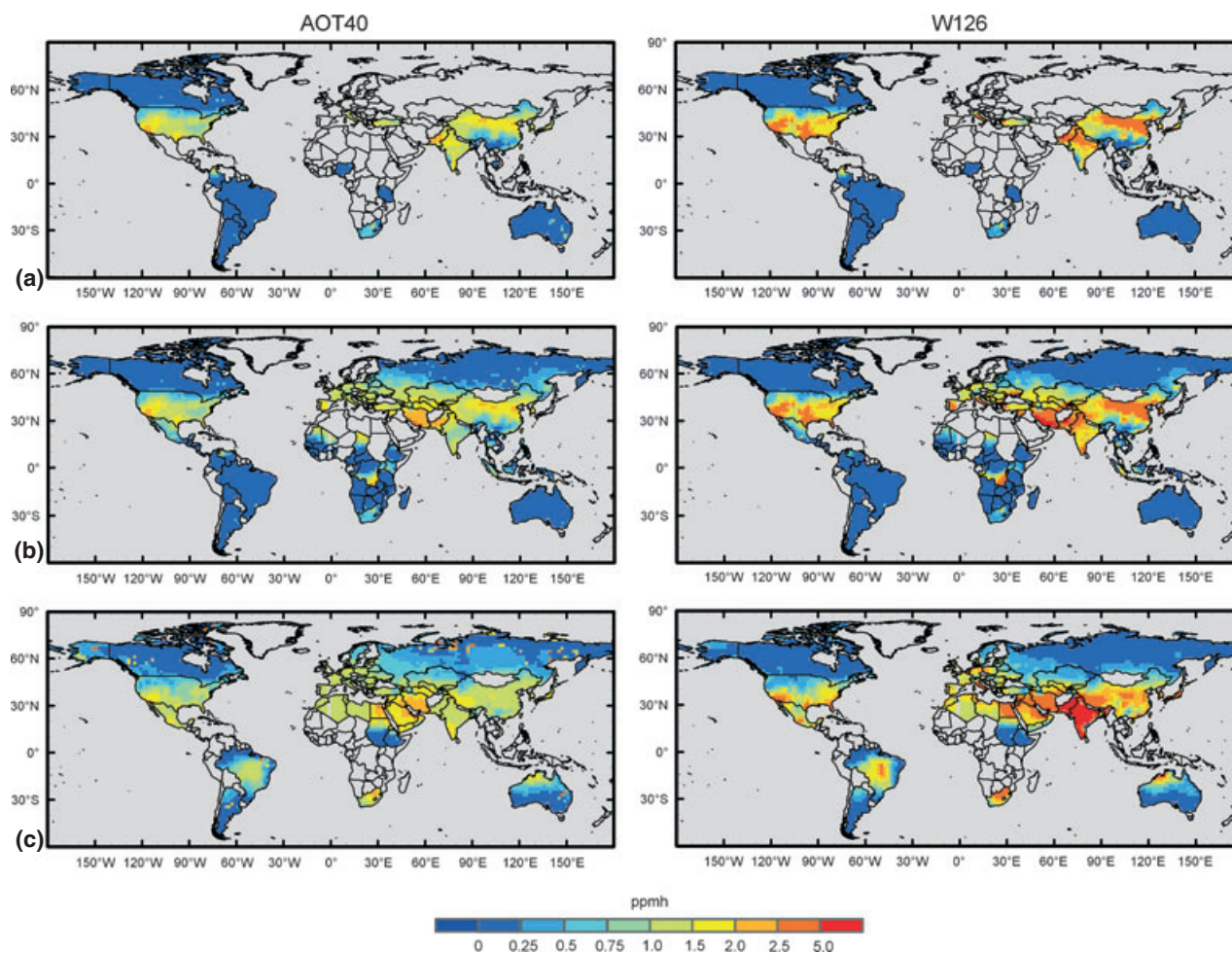
Fig. 1 Global distribution of the reduction in year 2030 O 3 exposure resulting from methane mitigation (CLE – CH 4 -red) according to AOT40 (left) and W126 (right) of (a) soybean, (b) maize, and (c) wheat during their respective growing seasons in each country (where crop calendar data are available). Minor producing nations not included in this analysis (where growing season data were unavailable) together account for <5% of global production of each crop (gray nations).
