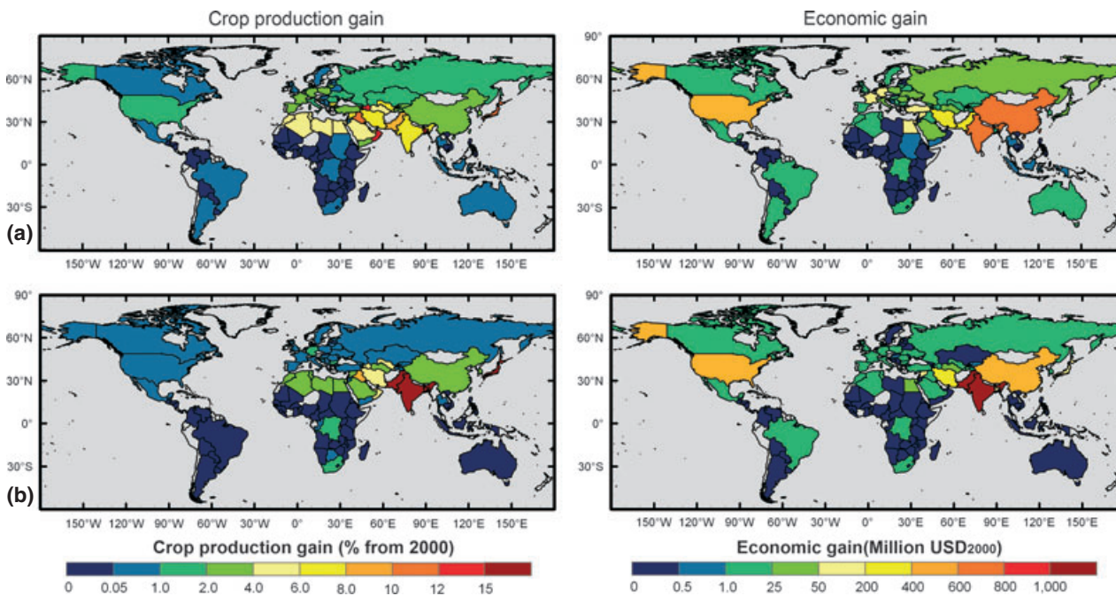
Fig. 2 Total (soybean, maize, and wheat) year 2030 crop production (CP) gain in each nation due to CH 4 mitigation as a percent increase from year 2000 production (left panels), and the estimated economic value (EV) of CP gains (right panels) according to (a) AOT40 and (b) W126. CP improvements represent the combination of estimated changes in O 3 concentrations during specific crop growing seasons in regions where crops are grown, and the quantity of each crop produced in each nation. EV values also reflect national producer prices in addition to these factors.
