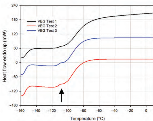
Figure 2 Changes in the heat capacity of VS. Differential scanning calorimeter thermograms during cooling ( a and b ) and warming ( c and d ) for VEG ( a and c ) as well as VED ( b and d ). Glass transition temperature ( T_g ) was extrapolated as the midpoint of the thermal transition during cooling. The absence of phase transition peaks during cooling and warming validates the lack of crystallization during cooling as well as devitrification and melting during warming for both VSs. Arrows indicate the onset of rapid warming at -110^\circ\text{C} , just above the temperature range of the glass transition.
