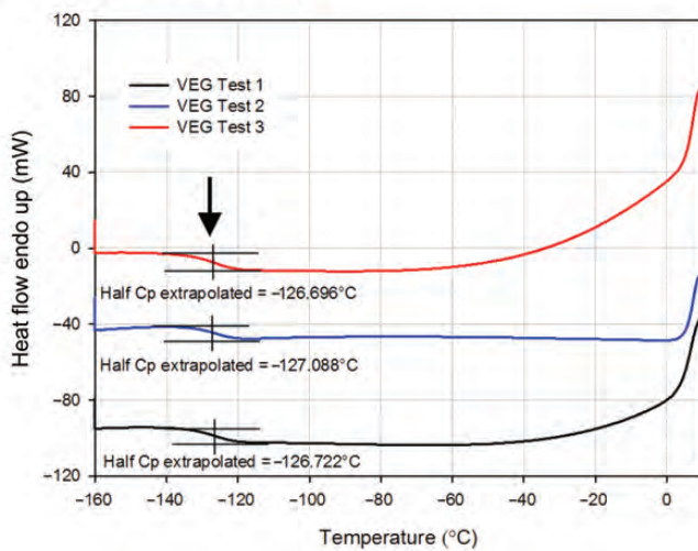
(c) VEG thermogram: warming
