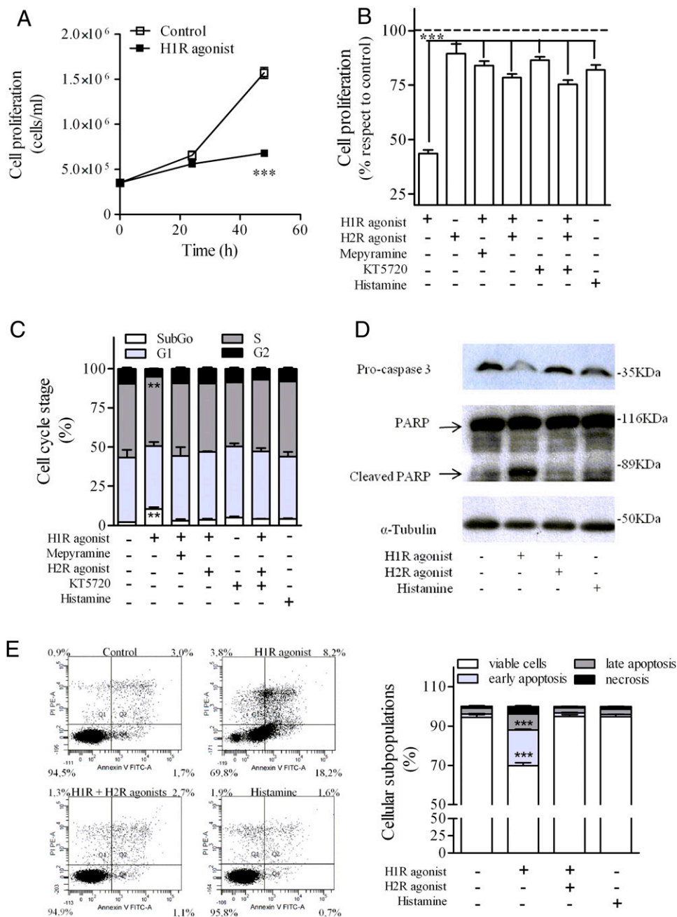
Fig. 4. Effect of H1R and H2R agonist on U937 cell proliferation and apoptosis. U937 cells were treated with 10 μM H1R agonist, 10 μM mepyramine, 10 μM H2R agonist, 10 μM KT5720, or 100 μM histamine alone or in combination for 24 and 48 hours (A) or 48 hours (B–E). After treatment, cell proliferation (A and B), cell cycle stage (C), pro-caspase 3 and PARP (D) and phosphatidylserine exposure at the cell surface by annexin V binding were evaluated as detailed in Materials and Methods . (A) Data were calculated as the means ± S.D. of assay triplicates. Similar results were obtained in at least three independent experiments. *** P ≤ 0.001 with respect to control cells. (B) Data represent mean ± S.E.M. ( n = 3). *** P ≤ 0.001 with respect to control cells. 100% corresponds to control cells. (C) Data were calculated as the means ± S.D. of assay triplicates. Similar results were obtained in at least three independent experiments. ** P ≤ 0.01 with respect to control cells. (D) Equal amounts of protein were subjected to SDS-PAGE and analyzed by Western blot with anti-caspase-3, anti-PARP, and anti-tubulin antibodies. (E) Different cell subpopulations according to the annexin V/PI staining pattern: Cells labeled with annexin V only were considered to be at an early apoptotic stage, cells labeled with annexin V and PI were considered to be at a late apoptotic stage, and cells labeled with PI only were considered necrotic. Data were calculated as the means ± S.D. of assay triplicates. Similar results were obtained in at least three independent experiments. *** P ≤ 0.001 respect to control cells.
