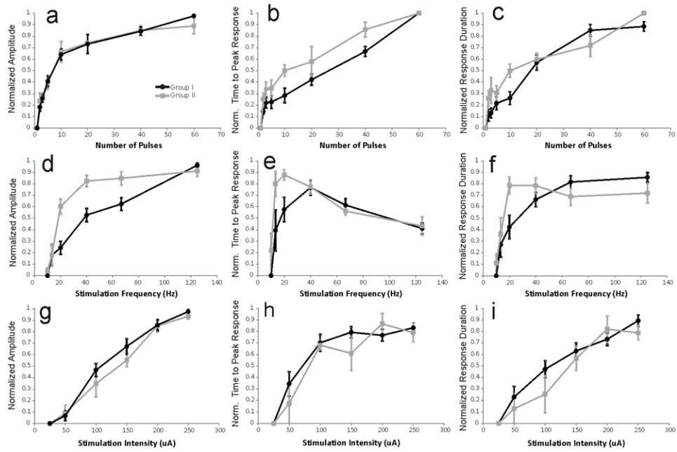
Figure 2. Group I (black lines, n=32 ) and Group II (gray lines, n=9 ) mGluR responses for different stimulation parameters. The first column represents the relationship between normalized mGluR amplitude and the number of stimulation pulses, stimulation frequency and stimulation intensity. The second column represents the relationship between normalized time-to-peak mGluR response and the number of stimulation pulses, stimulation frequency and stimulation intensity. The third column represents the relationship between normalized mGluR response duration and the number of stimulation pulses, stimulation frequency and stimulation intensity. With regard to Group I mGluR responses, data collected from VPM and layer 4 of S1 have been pooled together. Error bars represent SEM. Data were normalized using the value of the greatest response amplitude, time-to-peak, or duration, produced by each cell for each particular stimulation parameter (i.e. number of pulses, frequency, or intensity).
