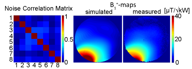
Figure 5. RF performance of the experimental hybrid applicator. Noise correlation matrix obtained for the decoupling of the 8 elements included in the proposed 8 channel TX/RX applicator (left). Simulated B_1^+ -map in [\mu\text{T}/\sqrt{\text{kW}}] derived from a single element; channel 5 in this case (middle). For this purpose a transversal slice through the center of the phantom was used. For comparison the measured B_1^+ -map is shown [\mu\text{T}/\sqrt{\text{kW}}] for the same slice and bow tie antenna element (right). doi:10.1371/journal.pone.0061661.g005
