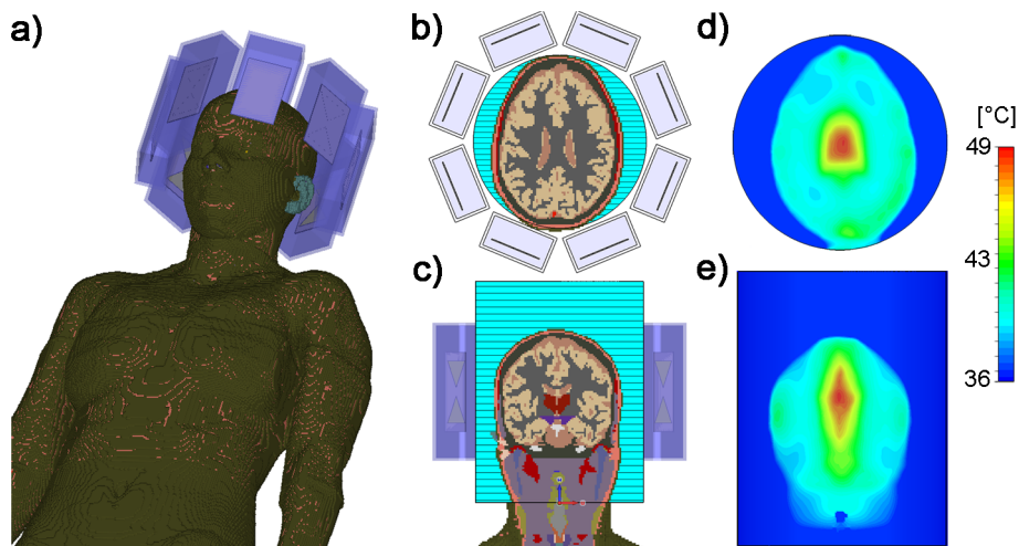
Figure 10. Simulation of RF heating in a human voxel model. Temperature simulations performed using the in vivo human voxel model “Ella” [37] in conjunction with the hybrid applicator. Positioning of the voxel model and eight bow tie dipole antennas (a). Axial and coronal slices through the human brain together with the dielectric medium adjusted to T=20^\circ\text{C} (b–c). Simulated temperature maps for a axial and coronal slice of the human brain (d–e). For this purpose RF heating was conducted over 5 min using an average RF power of 50 W per channel at 298 MHz. For the center of the brain the maximum temperature was 48.6^\circ\text{C} upon completion of the RF heating paradigm (d). In comparison the cranium’s surface did not exceed a temperature of 43.3^\circ\text{C} for the same heating paradigm.
