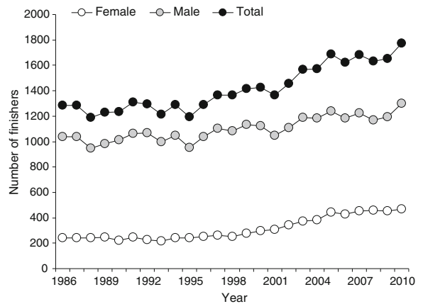
Fig. 1 Total number of finishers at the Hawaii Ironman Triathlon and number of finishers of each sex from 1986 to 2010
