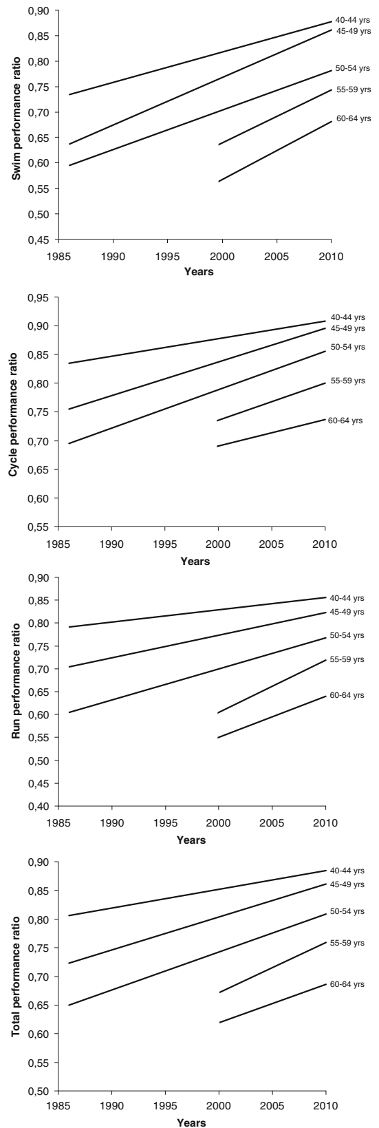
Fig. 4 Changes in performance ratios for swimming, cycling, running and total times by year for the top 10 finishers in each female age group. A performance ratio equal to 1 corresponded to the performance of the top 10 finishers of the 18–39-year age group. Solid lines represent conditions where the slopes of the linear regressions were significantly different ( P < 0.01 ) from zero. Dashed lines indicate the slopes of the linear regressions were not significantly different from zero. Lines traverse only the range of years for which data were considered
