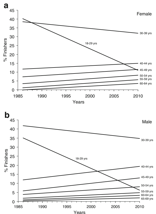
Fig. 2 Linear regressions defining the percentages of finishers within different age groups across the period of 1986 through 2010, for females (a) and for males (b). All the slopes of the linear regressions were significantly different ( P < 0.01 ) from zero
