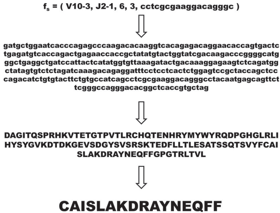
Figure 6. Once a sequence read has been classified according to the five variables described in the text, the underlying nucleotide sequence can be determined from the classifier, crucially without sequence error. From this underlying nucleotide sequence, it is then straightforward to determine the amino acid sequence via translation, where the CDR3 region is defined as the last conserved cysteine residue in V to the conserved FG(X)G motif in J.
