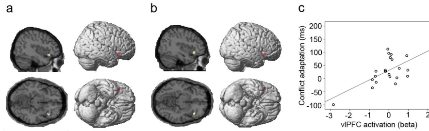
Figure 2. (a, b) Experiment 1 neuroimaging results for a whole-brain search for voxels displaying a positive correlation between conflict-driven neural activity and behavioral conflict adaptation scores, as defined by the previous \times current trial congruency interaction term ( [CI - CC] - [II - IC] ) (a), or as defined by the relative speed-up on incongruent trials only ( CI - II ) (b), are shown on sagittal and axial slices (left panels), and rendered (right panels), on a normalized brain (voxelwise height threshold = P < 0.005 , cluster extent threshold > 21 voxels). (c) Unbiased regression estimate (see Methods) of the association between inter-subject variability in behavioral conflict adaptation ( [CI - CC] - [II - IC] ) (y-axis) and conflict-driven activity in the right ventrolateral prefrontal cortex (vIPFC, x-axis).
