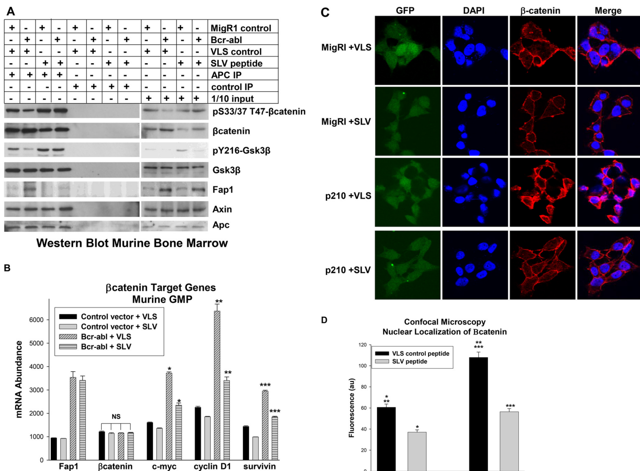
FIGURE 4. Bcr-abl influences \beta catenin expression and activity in a Fap1 -dependent manner in primary murine myeloid progenitor cells. A , treatment of Bcr-abl + primary murine myeloid progenitor cells with SLV peptide decreases Fap1 / Apc interaction, decreases tyrosine phosphorylation of Gsk3 \beta , decreases \beta catenin protein, and increases serine/threonine phosphorylation of \beta catenin. Bone marrow mononuclear cells from WT mice were transduced with a Bcr-abl -expression vector or empty control vector. The GMP population was cultured (as described above) and treated (IP) with Fap1 -blocking SLV peptide or control VLS peptide. Cell lysates were immunoprecipitated with an antibody to Apc or irrelevant control antibody, and immunoprecipitates were analyzed by Western blot analysis. Non-precipitated lysate was used to control for total protein abundance. Blots were serially probed with antibodies to total and serine/threonine phosphorylated \beta catenin, total and Tyr-216 phosphorylated Gsk3 \beta , Fap1 , Apc , and Axin . B , treatment of Bcr-abl + primary murine myeloid progenitor cells with SLV peptide decreases \beta catenin-target-gene expression. The cells described above were also analyzed for abundance of mRNA representing Fap1 , \beta catenin, and \beta catenin target genes ( c-myc , cyclinD1 , survivin ) by real-time PCR. Statistically significant differences in mRNA abundance with SLV versus VLS peptide are indicated by *, **, or ***. NS, not significant. C , SLV peptide treatment decreases nuclear \beta catenin in Bcr-abl + murine myeloid progenitor cells. Murine bone marrow cells were transduced with a Bcr-abl -expression vector or empty MigR1 control vector and treated with Fap1 -blocking SLV peptide or VLS control. Cells were analyzed by confocal microscopy for nuclear localization of \beta catenin. Transduced cells are green (green fluorescent protein label in vector), nuclei are indicated in blue (DAPI stain), \beta catenin is shown in red (Cy3-labeled secondary antibody), and purple indicates merged DAPI + Cy3 signals. D , nuclear \beta catenin is significantly decreased by SLV peptide treatment of Bcr-abl + murine bone marrow cells. The cells described above were analyzed for fluorescent intensity of the merged signal. At least 30 cells were counted in three fields for each sample. Statistically significant differences are indicated by *, **, or ***.
