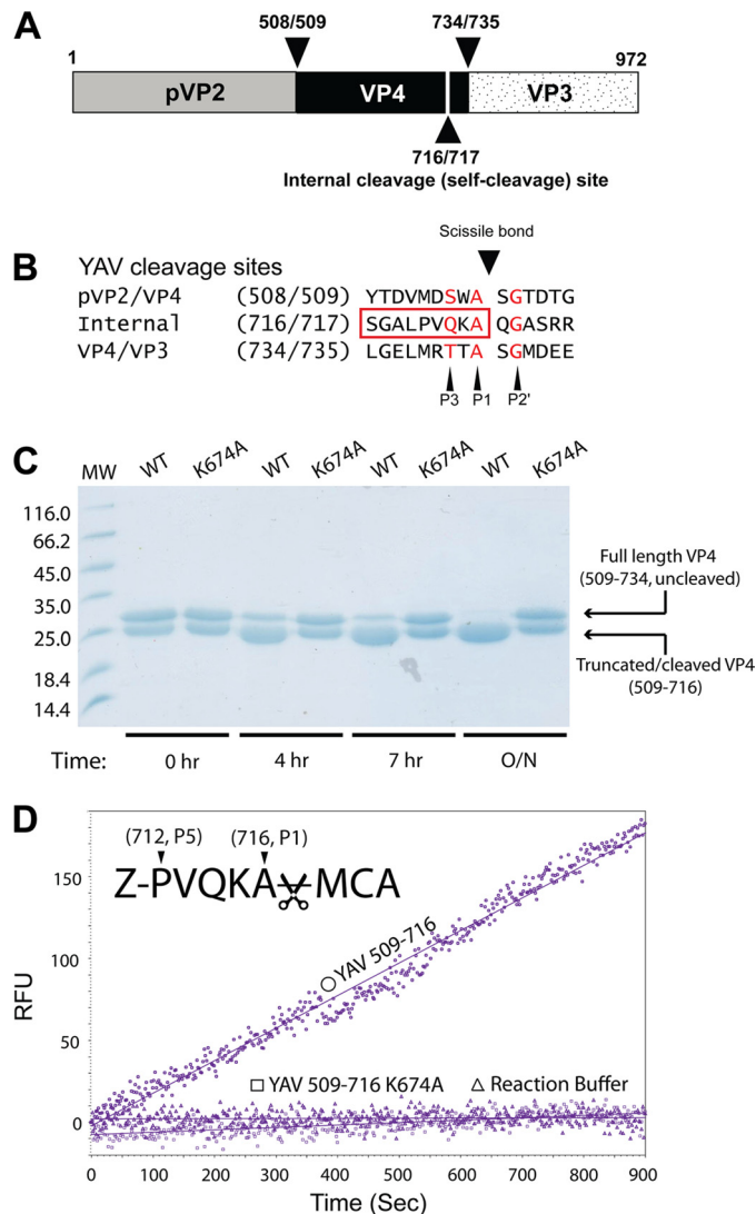
FIGURE 1. YAV VP4 protease truncated at the internal cleavage site is active. A, the genomic arrangement of segment A in YAV is shown. The major sites of cleavage are denoted by arrowheads with the P1 and P1' residue numbers listed. B, a list of known major YAV VP4 protease cleavage sites. The residues preceding P1' in the internal cleavage site are visible in the crystal structures and are boxed in red. C, to demonstrate processing at the internal cleavage site (after residue 716), truncated YAV VP4 (residues 509–716) was incubated with full-length YAV VP4 with an active site mutation (residues 509–734, K674A) for 0, 4, and 7 h and overnight at 23 °C. As a control, the same experiment was repeated with an enzyme with an active site mutation (residues 509–716, K674A). A 20- \mu l aliquot of the reaction was run on an SDS-polyacrylamide gel and visualized by Coomassie stain. D, a fluorometric peptide (benzyloxycarbonyl-PVQKA-4-methylcoumaryl-7-amide (Z-PVQKA-MCA)) corresponding to the sequence for residues P5–P1 of the YAV VP4 internal cleavage site (residues 712–716 of the YAV polyprotein) was incubated with truncated YAV VP4 (○; residues 509–716), truncated YAV VP4 active site mutant (□; residues 509–716, K674A) and reaction buffer (△; 20 mM MES, pH 6.5) alone. The relative fluorescence units (RFU; reduced values) are plotted over time.
