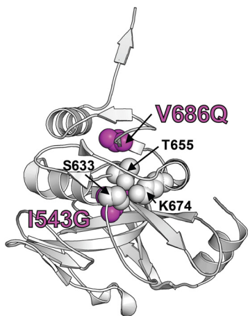
FIGURE 9. Mapping non-active site mutations that affect catalysis. The YAV VP4 active site residues are shown as spheres (Ser 633 , Lys 674 , and Thr 655 ). Polyprotein cleavage assays conducted by Imajoh et al. (24) have shown that non-active site mutations I543G and V686Q can significantly affect catalysis (shown as magenta spheres).
