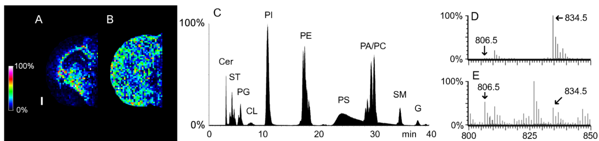
Fig. 4. Identification of MALDI-MSI species at m/z 806.5 and m/z 834.5 with the aid of ESI-LC-MS. MALDI-MSI rat brain images of the species m/z 806.5 (A) and m/z 834.5 (B) could each be either PS or ST species, or some combination of both. The white bar is 1 mm and the scale displays relative intensities with respect to the abundance of each ion. A total lipid extract of the serial section gives an ESI-LC-MS chromatogram (C) that separates PS and ST. LC-MS from the PS fraction (D) and ST fractions (E) show that 806.5 m/z is almost entirely ST (arrows) and 834.5 m/z is a mixture of PS and ST (arrows). MALDI-MS (Autoflex) and ESI-LC-MS (Q-TOF) spectra were acquired in negative mode.
