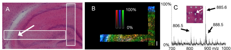
Fig. 6. Oversampling to improve the spatial resolution of MALDI-MSI. A: Optical image of an H&E stain of rat brain after MALDI-MSI analysis of the regions of interest within the white boxes. Mass Spectra were collected with oversampling in both 20 and 10 micron rasters across the hippocampal area. B: MALDI-MSI image of three molecular species displaying distribution across fine structures within the hippocampus. The white scale bar is 200 microns. Different color pixels represent different species, and stronger pixel intensities indicate greater abundance with respect to each ion. Green: m/z 885.5 representing PI(38:4); Blue: m/z 885.5 representing ST(d18:1/24:0); Red: m/z 1544.8 representing GM1(d18:1/18:0). C: MALDI mass spectrum approaching cellular resolution (location indicated with arrows in panel A and inset region). White marks on H&E section resulted from laser ablation of tissue at the center of each position. MSI images were acquired with an Autoflex in negative mode.
