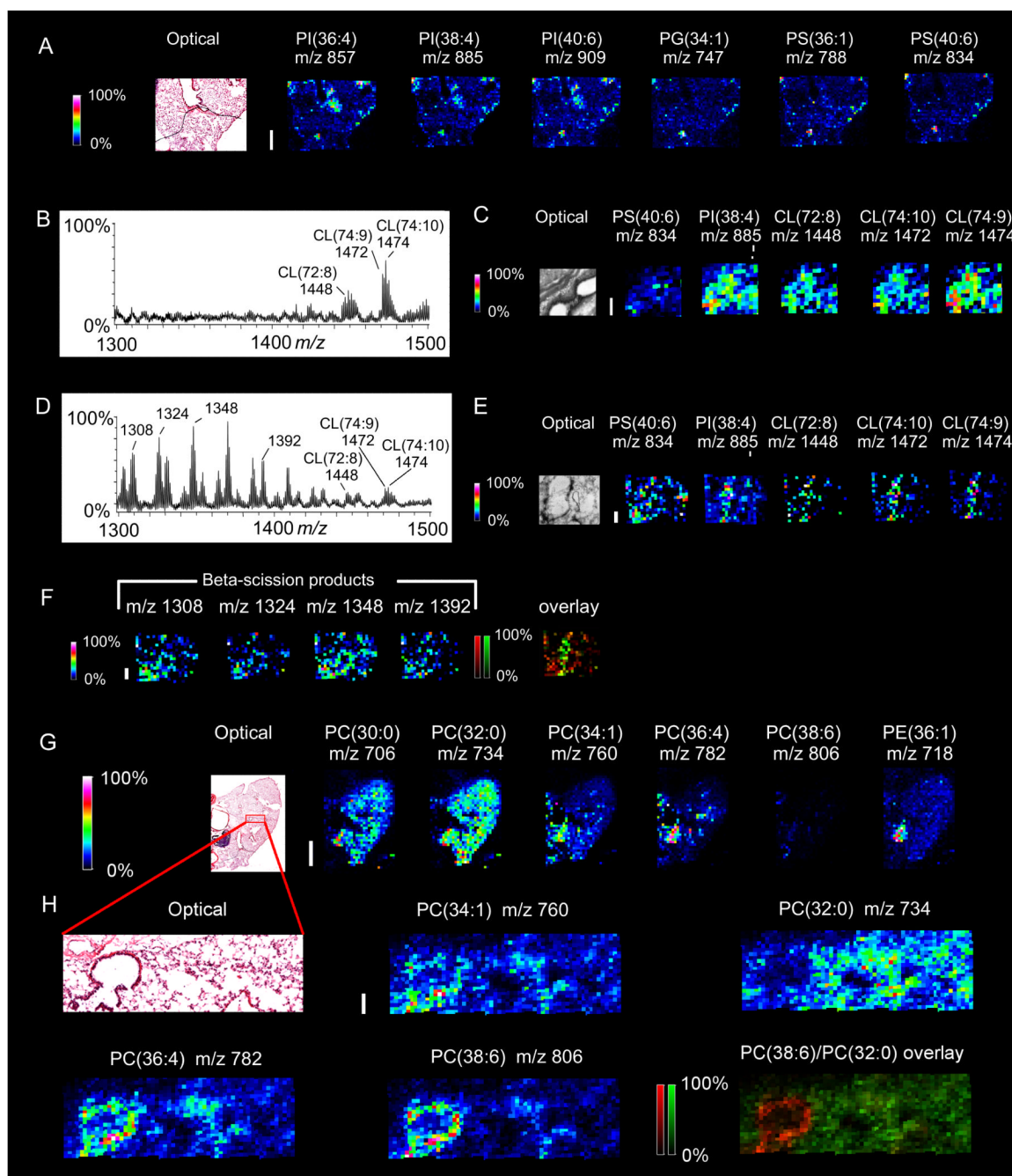
Fig. 8. MALDI-MSI of mouse lung determines regional assignment of critical common phospholipids and oxidation products of less abundant cardiolipin in acute lung injury (ALI). MALDI-MSI of normoxic lung in negative mode (A) detected several phospholipids but not cardiolipin. MALDI-MSI was performed at 50 micron spatial resolution and the white bar is 500 microns. Averaged MALDI spectra (B) and MALDI-MSI images (C) of lung tissue section treated with PLC from normoxic mouse detected CL clusters but not oxidative species of CL. MALDI-MSI was performed at 50 micron spatial resolution and the white bar is 200 microns. ALI-model mouse lung MALDI spectra (D) and MALDI-MSI images (E,F) in negative mode demonstrate decrease in CL content with detection of ions
