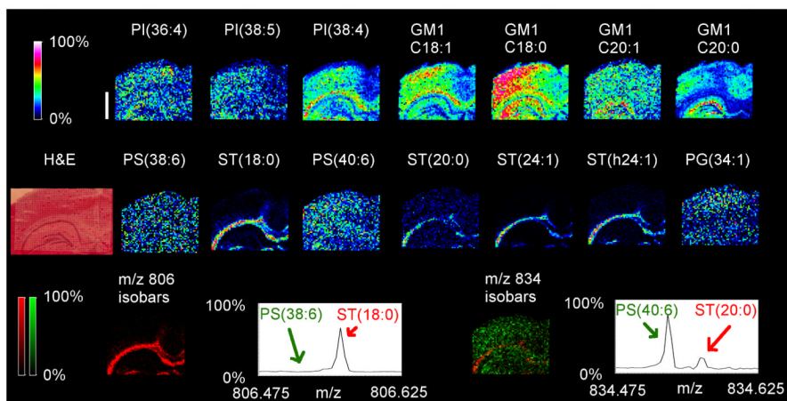
Fig. 5. FT-ICR MSI completely resolves isobaric rat brain species. Several lipid species from various classes were detected at high mass resolution and their localizations correlated with an H&E stain of the tissue section. The white bar is 1000 microns and the scale displays relative intensities with respect to the abundance of each ion. Two sets of isobaric species ( m/z 806.5 and 834.5) were completely resolved. The ions at m/z 806.497 and m/z 806.545 representing PS(38:6) and ST(d18:1/18:0) were resolved from each other, as were the ions at, m/z 834.528 and m/z 834.576 representing PS(40::6) and ST(d18:1/20:0), respectively. Each of these isobaric pairs was overlaid on the same MALDI image, but at the same absolute scale. Green pixels represented the PS species, and red represented the ST species. This confirmed that the m/z 806 species consisted almost entirely of ST(d18:1/18:0), while the m/z 834 species was mostly PS(18:0/22:6) but with a significant amount of ST(d18:1/20:0). The summation MALDI-MSI spectrum from the entire image further confirmed these results. MSI images were acquired with a Solarix in negative mode.
