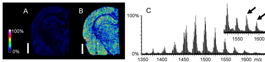
Fig. 7. MALDI-MSI of adult rat brain tissue after DHA supplementation. Heat-map MALDI-MSI of brains from naïve (A) and DHA-dosed (B) rats showed increase in the ion at m/z 834.5 which is partly composed of PS(18:0/22:6). The white bar is 2 mm and the heat map is scaled to relative intensities with respect to the abundance of the ion at m/z 834.5. Both images are presented at the same abundance scale. As such, 100% intensity represents the highest intensity observed between both images. LC-MS profiles of CL extracts from naïve (C) and DHA-dosed (inset) serial brain sections showed an increase in DHA-containing CL marked with arrows – m/z 1570: CL(18:0)(20:4)(22:6 \times 2); m/z 1592: CL(20:4 \times 2) (22:6 \times 2). Overall 29% of naïve and 38% of treated brain CL contained DHA. MALDI-MSI (Ultraflex II) and ESI-LC-MS (Q-TOF) spectra were acquired in negative mode.
