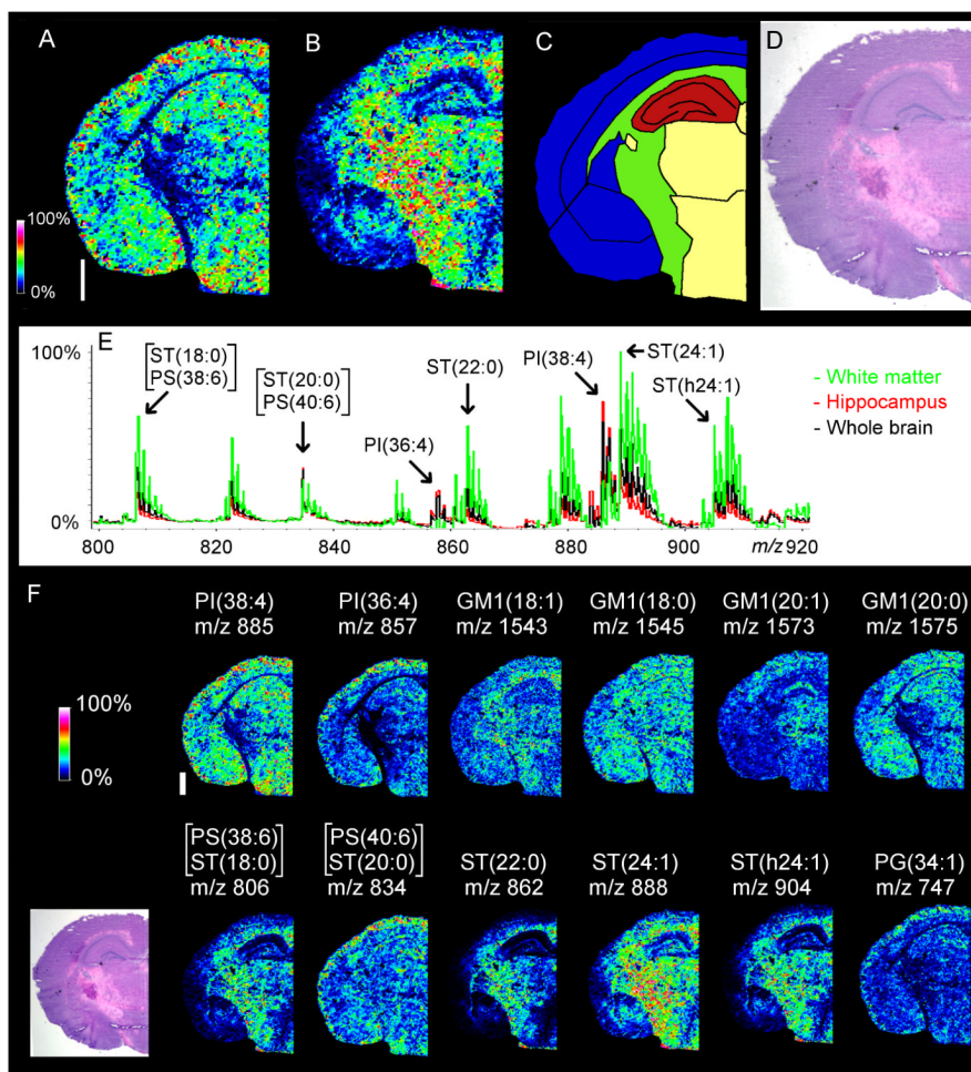
Fig 1. MALDI-MSI images and regional spectra of adult mouse brain. “Heat map” MALDI-MSI images of PI(38:4) ( m/z 885.5, panel A) and ST(24:1) with a d18:1 sphingosine ( m/z 888.5, panel B) display localization to different regions of the brain. The white bar is 1000 microns and the scale displays relative intensities with respect to the abundance of each ion. These lipids correlate to specific brain structures (C) upon comparison with a serial H&E section (D). Comparison of the averaged MALDI-MSI spectrum from the entire tissue slice (E - black trace) with that of the hippocampus (E - red trace) and white matter (E - green trace) shows that many other d18:1 sulfatide species including ST(24:1) are more abundant in the white matter than the hippocampus, while the opposite is the case with several PI species including PI(38:4). Various lipids from several classes were also detected (F). Several species of ganglioside GM1 with d18:1 sphingosines exhibited different localization, depending on the composition of their long chain base. MALDI-MSI images were acquired in negative mode with an Ultraflex II.
