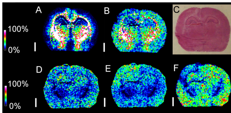
Fig. 9. MALDI-MSI of pnd 17 rat brain after trauma. MALDI-MSI in negative mode shows different distributions of m/z 806.5 that contains nonoxidizable ST(d18:1/18:0) (A) and m/z 834.5 that contains oxidizable PS(18:0/22:6) (B) in brain after controlled cortical impact. Region of damage is shown by an arrow on serial H&E (C). The white bar is 200 microns and the scale displays relative intensities with respect to the abundance of each ion. While m/z 806.5 was detected in similar abundances between the hemispheres ipsilateral and contralateral to the point of impact, m/z 834.5 is somewhat reduced in the ipsilateral cortical and hippocampal regions with respect to the contralateral regions. MALDI-MSI in positive mode detected different abundances of PC(16:0/16:0) adducts between both hemispheres. While the [M+H]^+ ion at m/z 734.5 (D) was detected in similar abundance ipsilateral and contralateral, the [M+Na]^+ adduct ion at m/z 756.5 (E) was in greater abundance ipsilateral while the [M+K]^+ adduct ion at m/z 772.5 (F) was in greater abundance contralateral. Negative mode and positive mode MSI images were acquired with an Autoflex.
