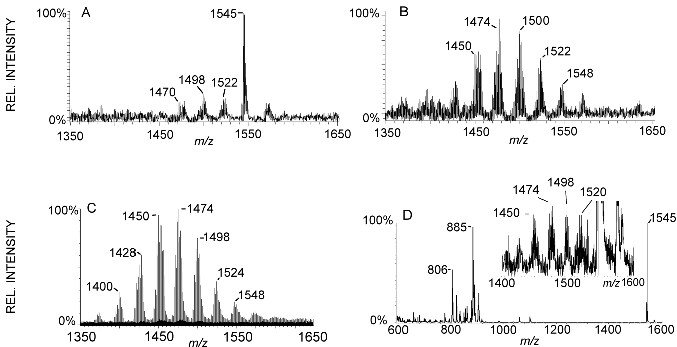
Fig 2. Comparison MALDI-MS and ESI-LC-MS from pnd 17 rat brain. A: MALDI-MS of brain total lipid extract barely detects some CL species predominantly as [M-2H+Na]^- adducts. Ganglioside GM1 at m/z 1545 obscures CL in this region. B: Split-flow LC-MS allowed collection of this CL fraction and subsequent analysis by MALDI-MS resulting in more species of CL detected, and these were mixtures of [M-H]^- and [M-2H+Na]^- adducts. C: ESI-LC-MS of same total lipid extract detects 70 species of CL, and these were detected as [M-H]^- ions. D: On-tissue phospholipase C (PLC) treatment and subsequent washing results in MALDI-MSI detection of several species of CL predominantly as [M-H]^- ions. The inset region is at 50 \times magnification. MALDI-MS and -MSI were acquired with an Autoflex in negative mode and ESI-LC-MS with a Q-TOF in negative mode.
