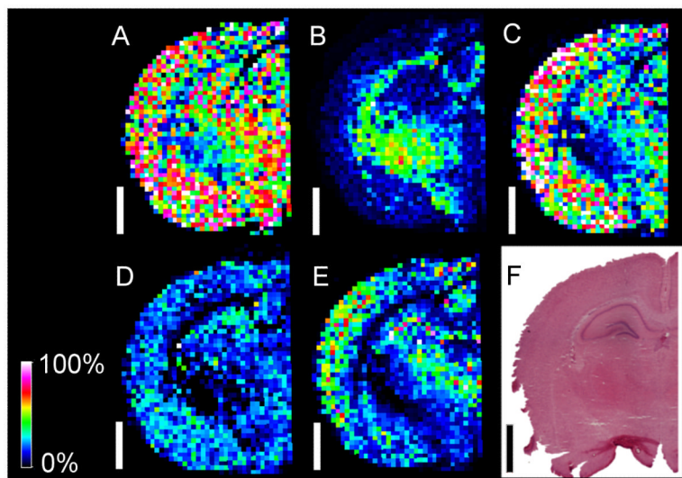
Fig. 3. MALDI-MSI of cardiolipin (CL) and other more abundant phospholipids after on-tissue phospholipase C (PLC) treatment. The white bar is 2mm and the scale displays relative intensities with respect to the abundance of each ion. A: PI(38:4) m/z 885.5, B: ST(24:1) m/z 888.5, C: GM1(d18:1/18:0) m/z 1544.8; D: CL(72:8) m/z 1447.9, E: CL(74:7) m/z 1477.9, F: near-serial H&E section. MSI images were acquired with an Autoflex in negative mode.
