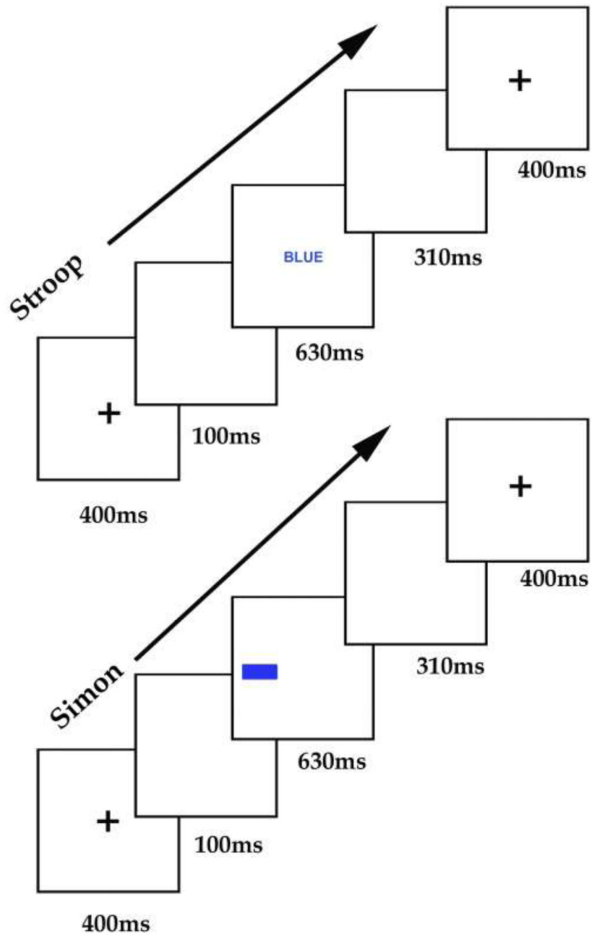
Figure 3. Illustration of Stroop and Simon paradigms
