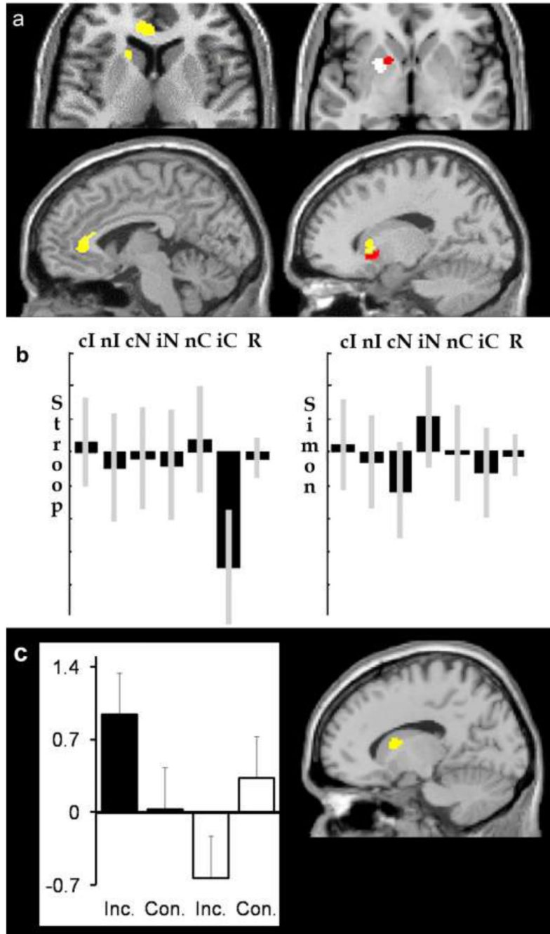
Figure 5. Activation change for controlling interference
