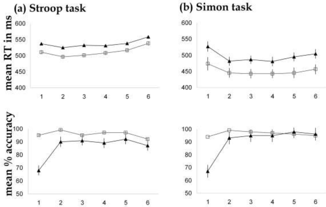
Figure 4. In-scanner behavioral data
