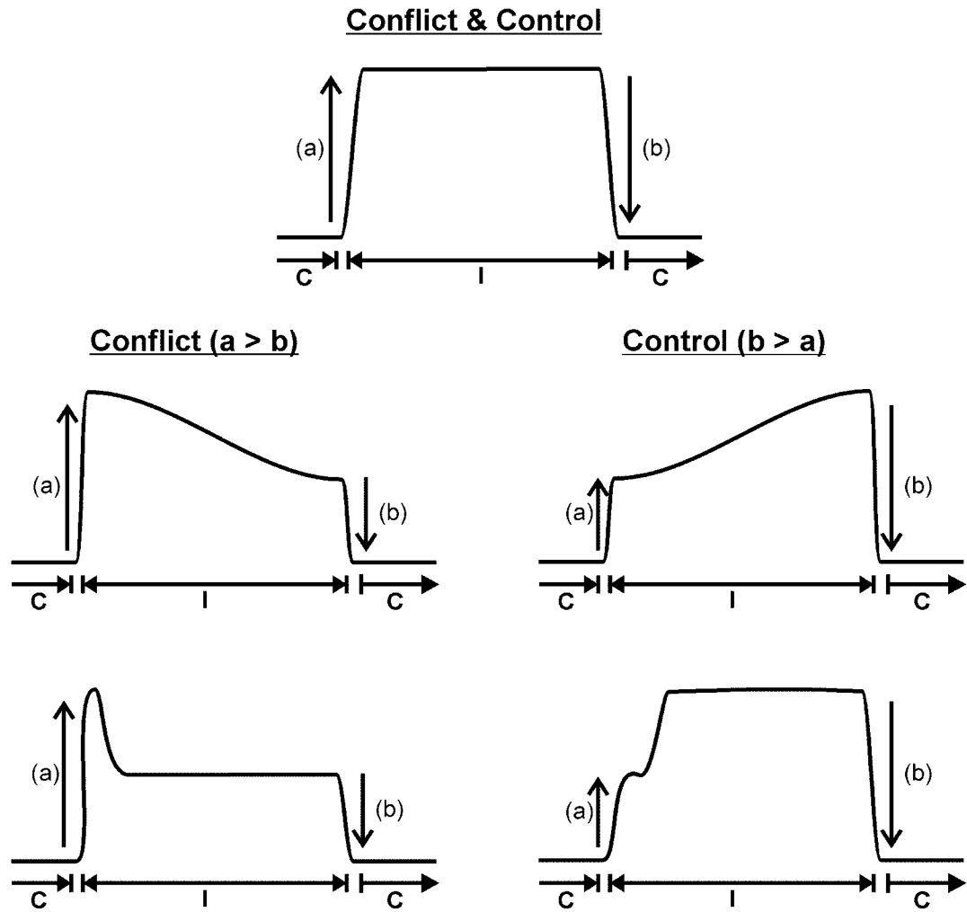
Figure 1. Predictions for activation related to conflict and its control during incongruent trials Top shows expectation that activation related to conflict and control will (a) increase at the start of a run of incongruent trials and (b) decrease at the end of a run of incongruent trials. C = run of congruent trials. I = run of incongruent trials. Lower two rows show the differing expectations for conflict and control. The expectation is that conflict will be higher at the start of a run of incongruent trials than the end of a run of congruent trials, i.e., (a) will be greater than (b). In contrast, control is expected to be higher at the end of a run than the beginning of the run, i.e., (b) will be greater than (a). The shape of these effects across an incongruent run could either be gradual (middle row) or primarily occur on the second run of a trial and then plateau for the rest of the run (lower row). The changing effect of control during a congruent or neutral run could also be gradual or stepwise, however, our experimental design and analysis do not allow us to determine how activation related to control changed over trials of the same type.
