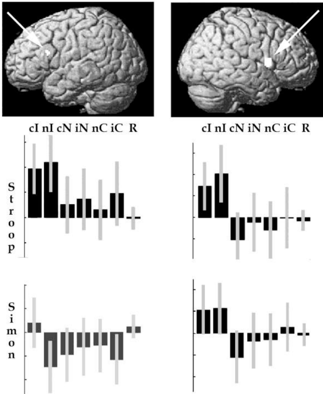
Figure 6. Activation change for the onset of interference
