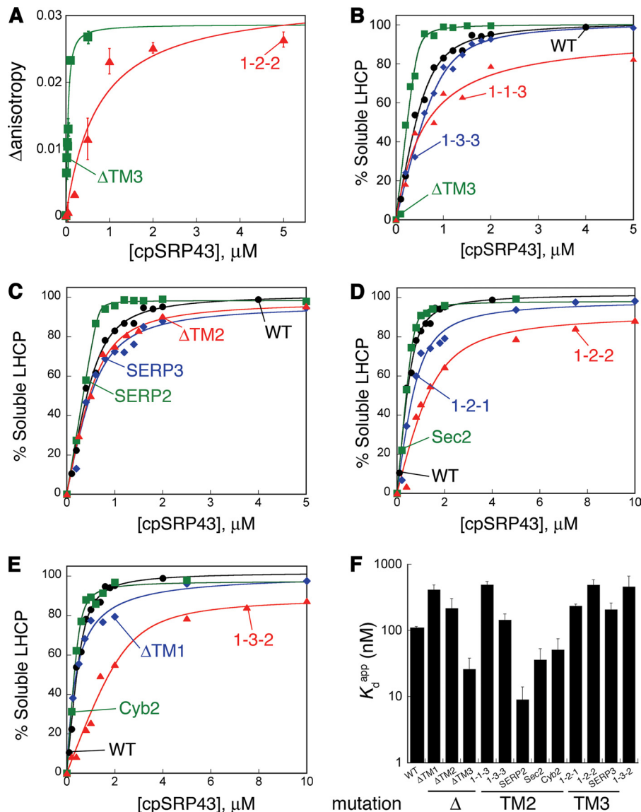
FIGURE 2. cpSRP43 can interact with a variety of LHCP TM mutants. A , binding of cpSRP43 to TM mutants as measured by changes in anisotropy. Fits of data gave K_d values of 22 nM for \Delta TM3 and 713 nM for 1-2-2. For comparison, the K_d^{app} values measured by light scattering were 26 and 489 nM, respectively (Table 4). B–E , binding of cpSRP43 to LHCP and its TM mutants as measured by the ability of cpSRP43 to prevent the aggregation of substrate proteins (see “Experimental Procedures”). The data were fit to Equation 1 (see “Experimental Procedures”) and gave K_d^{app} values that are summarized in Table 4. F , summary of the K_d^{app} values of all the LHCP TM mutants characterized in this study. Values of K_d^{app} were determined by a combination of light scattering and fluorescence anisotropy assays.
