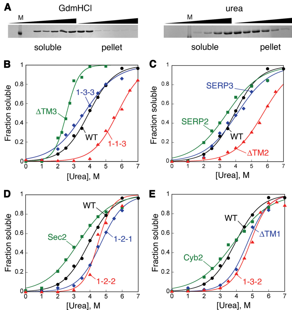
FIGURE 7. The irreversible TM mutants form ultrastable aggregates. A , sedimentation analysis of the ability of guanidinium chloride ( GdmHCl ) and urea to resolubilize LHCP aggregates. M denotes the protein marker lane. B–E , urea solubilization curves of LHCP and its TM mutants. The data were fit to Equation 8 (see “Experimental Procedures”) and gave U_{50} values (Table 4).
