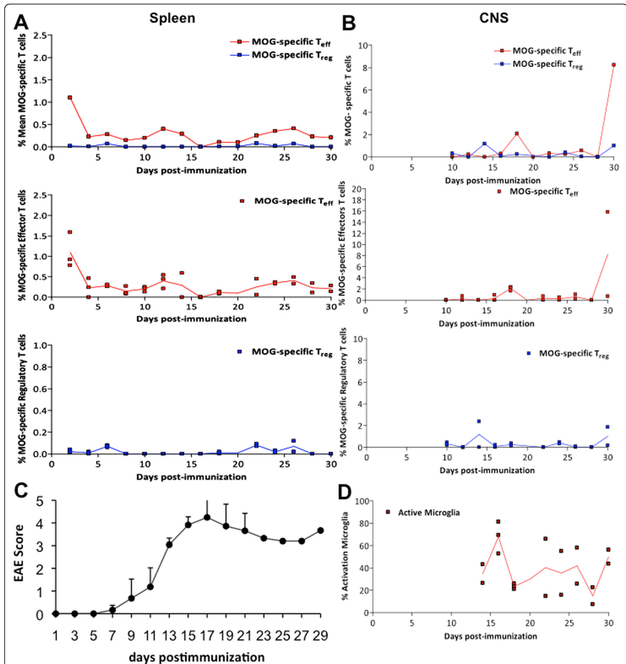
Figure 5 Dynamics of activated MOG-T eff , MOG-T reg cells and microglia in secondary lymphoid organs and CNS during the course of EAE after B cell depletion. A ) Percentage of MOG-specific T eff (red) or T reg (blue) cells in the spleen after immunization. The upper graph shows the mean of measurements from 3 animals each day, and the bottom panels show the distribution of all measurements for each subpopulation as dots, with the mean in black; B ) percentage of MOG-specific T eff (red) or T reg (blue) cells in the CNS from day 9 after immunization. The upper graph shows the mean of measurements from 3 animals each day, and the bottom panels show the distribution of all measurements for each subpopulation as dots, with the mean in black; C ) clinical score of animals suffering EAE after B cell depletion (mean + SD); D ) percentage of activated microglia in the CNS from day 9 after immunization.
