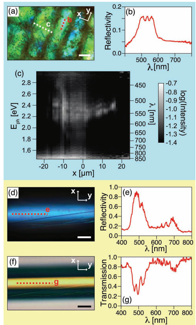
Figure 2. Optical characterization of the fruit and the fibers. (a) Optical micrograph of a fruit's surface visualizing parts of elongated tissue cells. (b) The corresponding reflection spectrum averaged along the red dashed line in (a). (c) Spectrally resolved intensity distribution acquired from a line scan (white dashed line in (a)) radially across a single cell showing the variation of the reflection band induced by the curvature of the layered nanoscale architecture. E_{ph} - photon energy, x - spatial position radially along the fiber, centered at the fiber axis. (d) Optical micrograph of a blue fiber in reflection. (e) The corresponding reflection spectrum averaged along the red dashed line in (c). (f) Optical image of the same fiber in transmission. (g) The corresponding transmission spectrum averaged along the red dashed line in (e). All scale bars: 20 \mu\text{m} .
