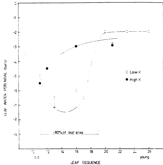
FIG. 4. Leaf water potentials determined by the Shardakov technique for various blades of K deficient (low K) and K sufficient (high K) plants. Arrows on points indicate true values were greater than ( \uparrow ) or less than ( \downarrow ) the value shown.
