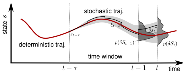
Figure 1. The time window and the error propagation dynamics used for calculating the TiPI, eq. (11). In principle, the process is considered many times with always the same starting value but different realizations of the noise \xi . Note that, when using the one-shot gradients, only one realization is needed. doi:10.1371/journal.pone.0063400.g001
