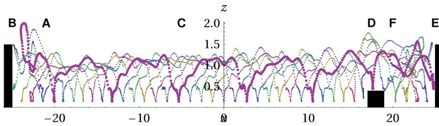
Figure 7. Regular locomotion pattern and interaction with the environment. Plotted are the center positions of the 6 rigid segments in space for an interval of 40 sec. One line is highlighted for visibility. The trajectory starts while the robot is moving to the left (A) and is hitting the wall (B) (black box) and locomotes to the right (C) showing a very regular pattern. Then it overcomes an obstacle (D) and hits the wall (E) and moves back (F). The behavior is cyclic. Parameter: \varepsilon = 0.005 . doi:10.1371/journal.pone.0063400.g007
