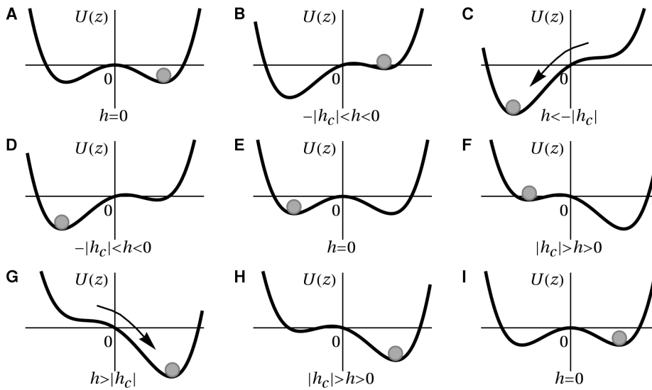
Figure 2. The hysteresis cycle in the gradient picture. The diagrams show the stages of one hysteresis cycle starting from h=0 (A) with the state at z>0 as represented by the sphere. Decreasing h creates the asymmetric situation (B). If h = -h_c the saddle-node bifurcation happens, i. e. both the maximum at z=0 and the right minimum disappear so that the system shifts to the left minimum (C). Increasing h until h=0 brings us back to the initial situation with the state shifted to the other well see (D,E). The diagrams (F) and (G) depict the switching from the minimum at z<0 to the minimum at z>0 by increasing h . By decreasing h until h=0 the hysteresis cycle is finished, see (H,I). doi:10.1371/journal.pone.0063400.g002
