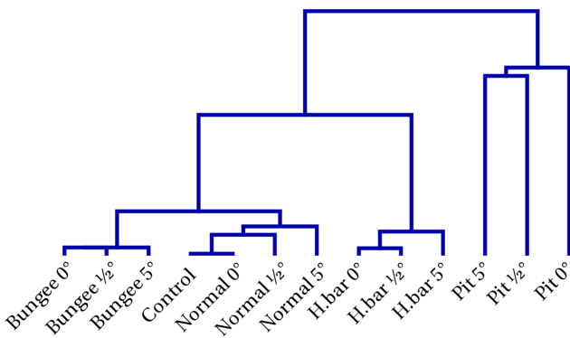
Figure 10. Parameter similarity for the behavior in different environments (Fig. 9). Plotted is the results of a hierarchical clustering based on the difference between the parameters in each of the simulations (averaged over time). For each of the four environments there are three initial poses: 0° (straight upright), 0.5° and 5° slanted to the front. The parameters for runs in the same environment are clustered together. This supports the observation that the embodiment plays an essential role in the generation of behavior. More importantly the physical conditions are reflected in the parameters and are thus internalized. We used the squared norm of the difference of the absolute values of the matrix elements. The absolute values were used because a common structure in the parameters are rotation matrices and there the same qualitative behavior is obtained with inverted signs. Parameters: \varepsilon = 10^{-5} , \eta = 0.005 , update frequency 50 Hz. doi:10.1371/journal.pone.0063400.g010
