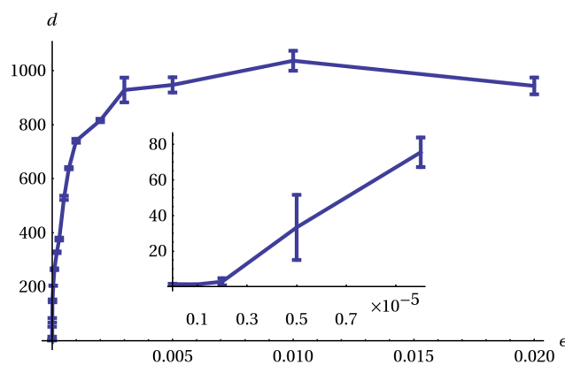
Figure 6. Role of the fast synaptic dynamics: depending on the speed of the synaptic dynamics defined by \varepsilon , the locomotion properties are changing drastically. Depicted is the distance traveled by the robot in 10 min simulated time on an empty plane. The inset gives a close up view for low \varepsilon , demonstrating that the locomotion starts only if \varepsilon exceeds a certain threshold value. Shown is the mean and standard deviation of 10 runs each. Update frequency 25 Hz. doi:10.1371/journal.pone.0063400.g006
