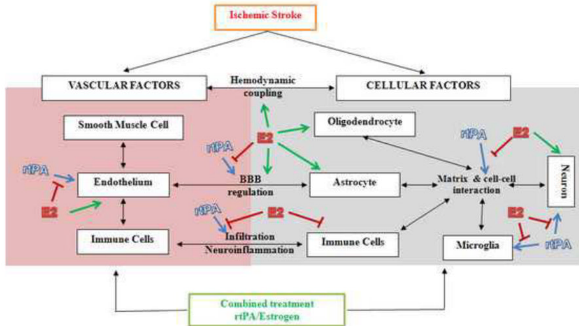
Figure 1. Schematic presentation of the potential mechanisms underlying the combined rtPA/estrogen treatment for ischemic stroke
