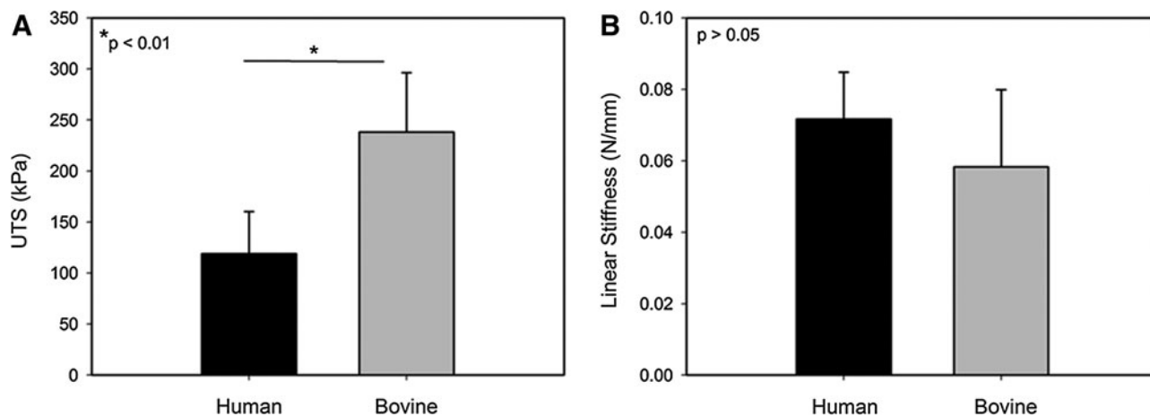
FIG. 6. Mechanical properties of 12 wt./vol.% electrospun collagen scaffolds fabricated using bovine-derived or plant-derived human collagen. (A) UTS is significantly greater in bovine scaffolds; however, no statistical difference was found in linear stiffness (B).
