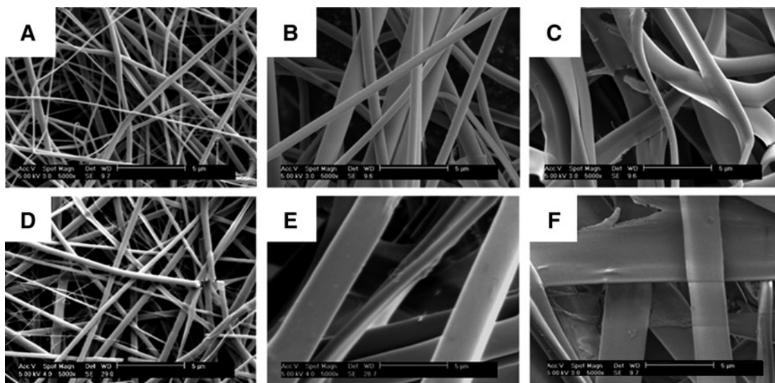
FIG. 4. Fibrous collagen scaffolds fabricated via electrospinning of plant-derived human (A–C) or bovine collagen (D–F). Electrospun scaffolds were spun using (A, D) 12, (B, E) 16, and (C, F) 20 wt./vol.% solutions of collagen in hexafluoroisopropanol. Fibrous human collagen scaffolds were characterized by thinner, more uniform rounded fibers. In contrast, bovine collagen fibers exhibited ribbon-like morphologies at concentrations greater than 12 wt./vol.%. Scale bar = 5 \mu m.
