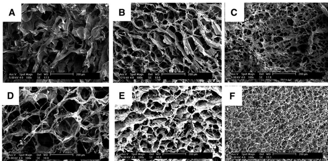
FIG. 1. Collagen sponges fabricated via lyophilization of a 0.6 wt./vol.% solution of plant-derived human (A–C) or bovine collagen (D–F) in 0.5M acetic acid. Casting frames were frozen in -20^{\circ}\text{C} air [slow; (A, D)], -80^{\circ}\text{C} air [medium; (B, E)], or -80^{\circ}\text{C} ethanol [rapid; (C, F)]. Scale bar = 200 \mu\text{m} .
