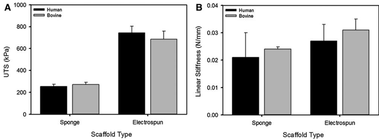
FIG. 11. (A) UTS and (B) linear stiffness of engineered skin at culture day 14 as a function of the scaffold type and source material.
