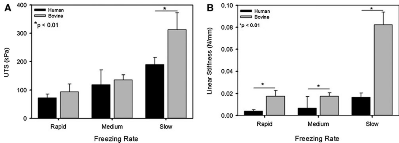
FIG. 3. Mechanical properties of acellular collagen sponges fabricated using plant-derived human or bovine collagen. (A) Ultimate tensile strength (UTS) is significantly greater in large pore size bovine sponges with no statistical difference measured between small or medium bovine or human collagen sponges. (B) Bovine collagen sponges were observed to be stiffer in each freezing condition.
