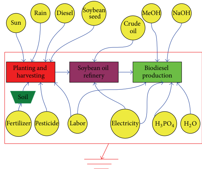
FIGURE 5: Emergy flow diagram of soybean-based biodiesel production system.
