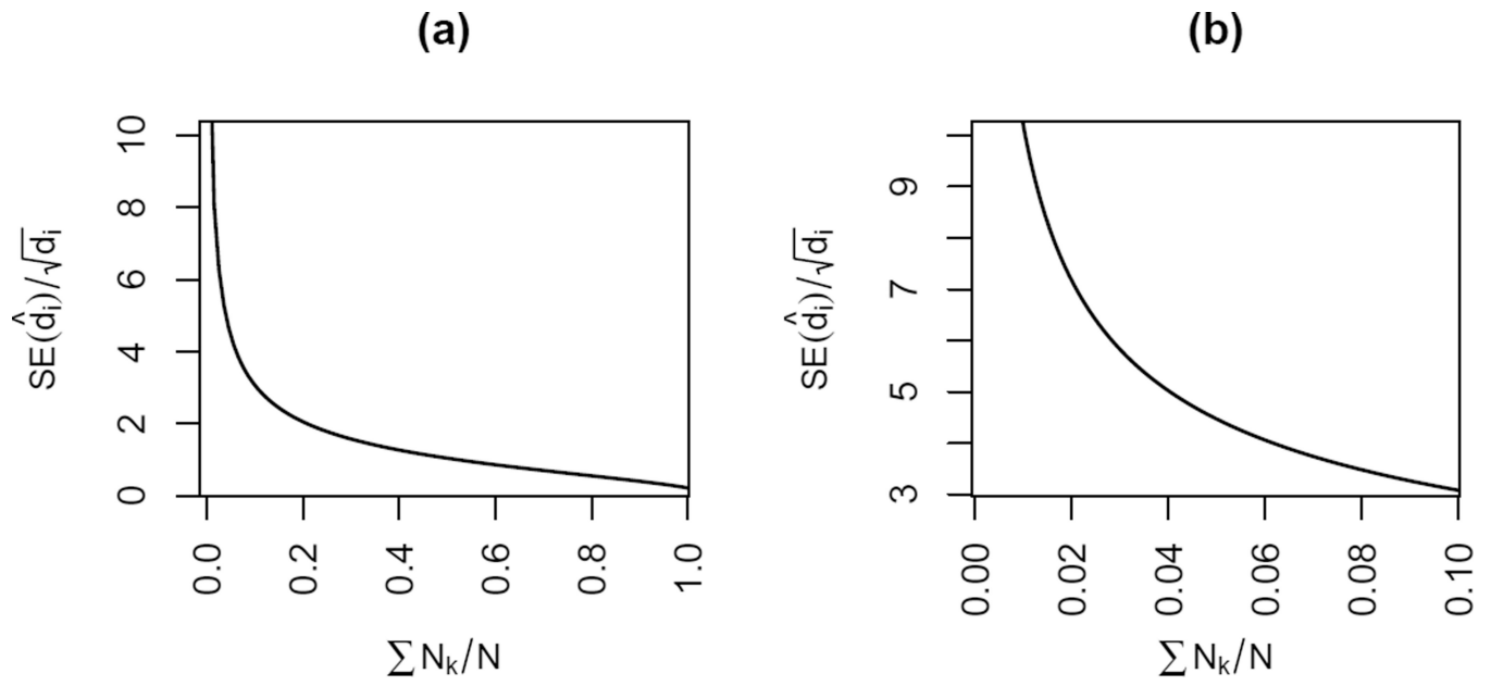
Figure 1. Standard error of the simple scale-up degree estimate (scaled by the square root of the true degree) plotted against fractional subpopulation size. As we increase the fraction of population represented by survey subpopulations, the precision of the estimate improves, with diminishing improvements after about 20%.
