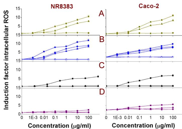
Fig. 7. DCFH-DA assay on NR8383 and Caco-2 cells after 24 h exposure to (A) Si(1.6) NP-NH 2 (■), Si(1.6) NP-N 3 (▲) and Si(1.6) NP-COOH (●); (B) SiFe(3.9) NP-NH 2 (■), Si(3.9) NP-NH 2 (▲), SiMn(3.9) NP-NH 2 (●), SiFe(3.9) NP-NH 2 -Dex (□), Si(3.9) NP-NH 2 -Dex (▲) and SiMn(3.9) NP-NH 2 -Dex (●); (C) Ge NP-TMPA (■), Ge NP-PEG (▲) and Si NP-PEG (●); (D) Si NP-Sil (■), Si NP-UDA (▲) and Si NP-Pol (●). Results are shown as mean ± SEM (n = 3).
