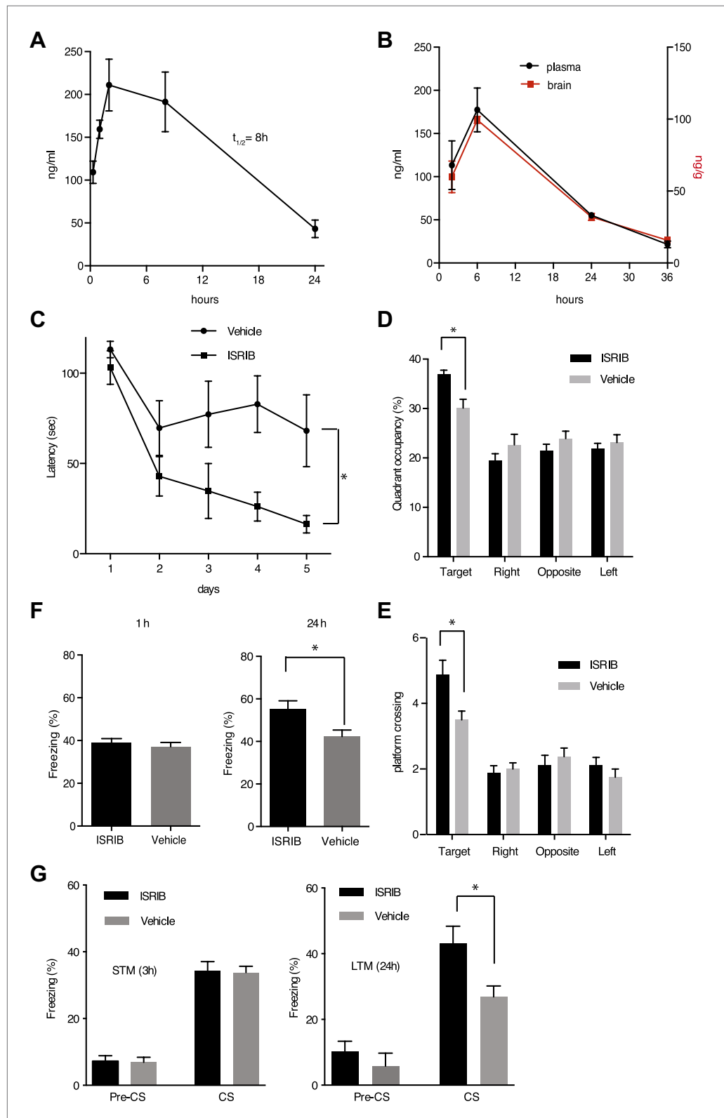
Figure 6. ISRIB enhances spatial and fear-associated learning in rodents. (A) Plasma concentration (ng/ml) of ISRIB after a single intraperitoneal injection (5 mg/kg). Plasma was collected at the indicated times and the concentration was determined by mass spectrometry (mean \pm SEM, N = 3). (B) Brain (ng/g tissue) and plasma concentrations (ng/ml) of ISRIB after a single intraperitoneal injection (2.5 mg/kg). Data (mean \pm SEM, N = 3) were obtained at the Figure 6. Continued on next page
