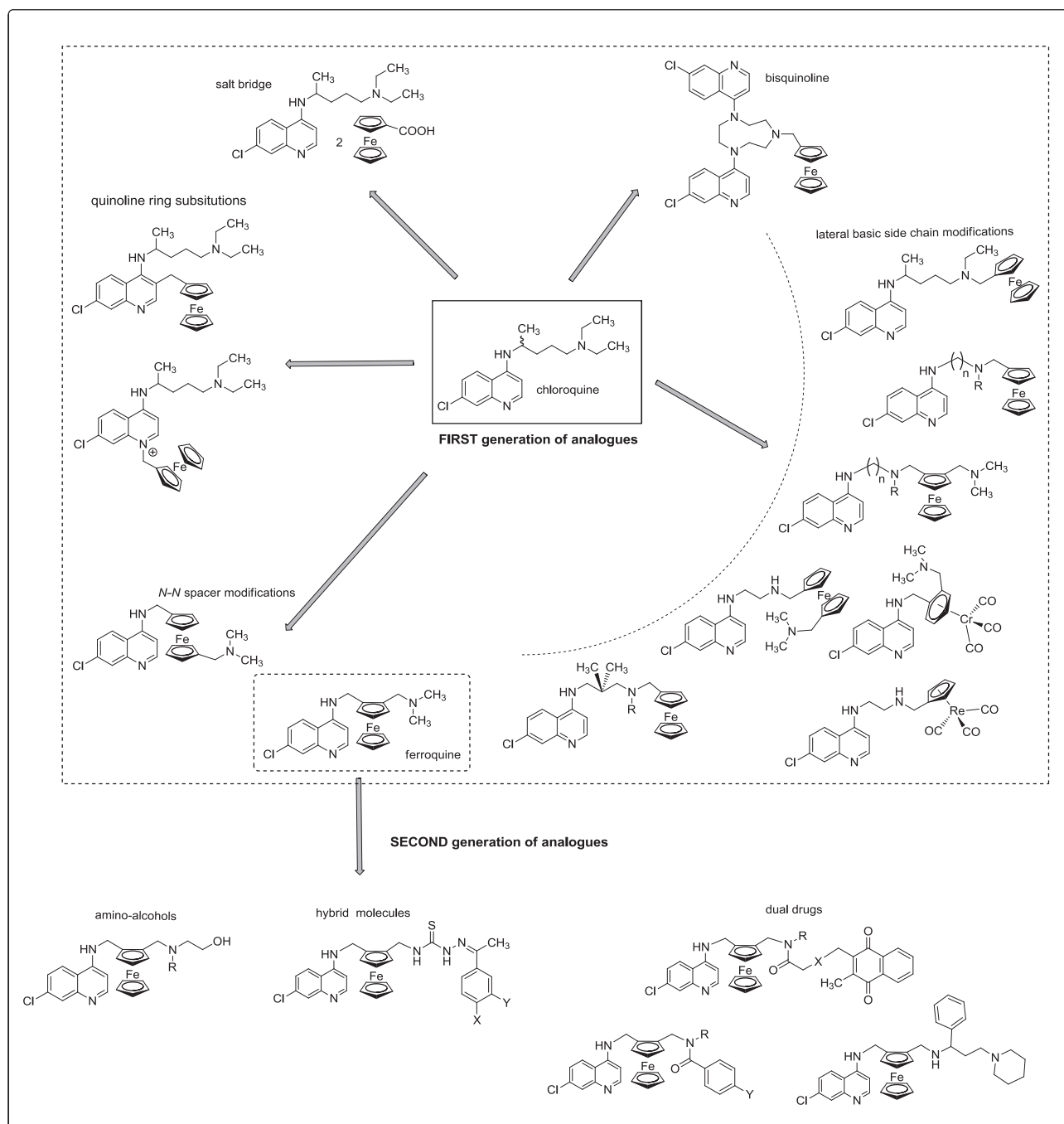
Fig 1. – Scheme of different strategies adopted in synthesis of ferrocene-CQ hybrids.
