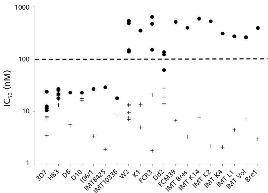
Fig 2. – Susceptibility of 19 laboratory P. falciparum clones to CQ and FQ compiled from 11 different published studies.
