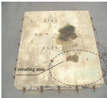
FIGURE 3: General view of concrete slab specimen.
