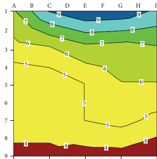
FIGURE 7: Contour plot of concrete resistivity \rho .
