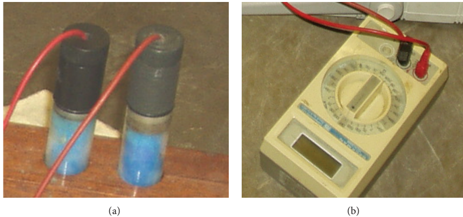
FIGURE 4: Half-cell potential measurements: (a) copper/copper sulphate electrode and (b) digital voltmeter.
